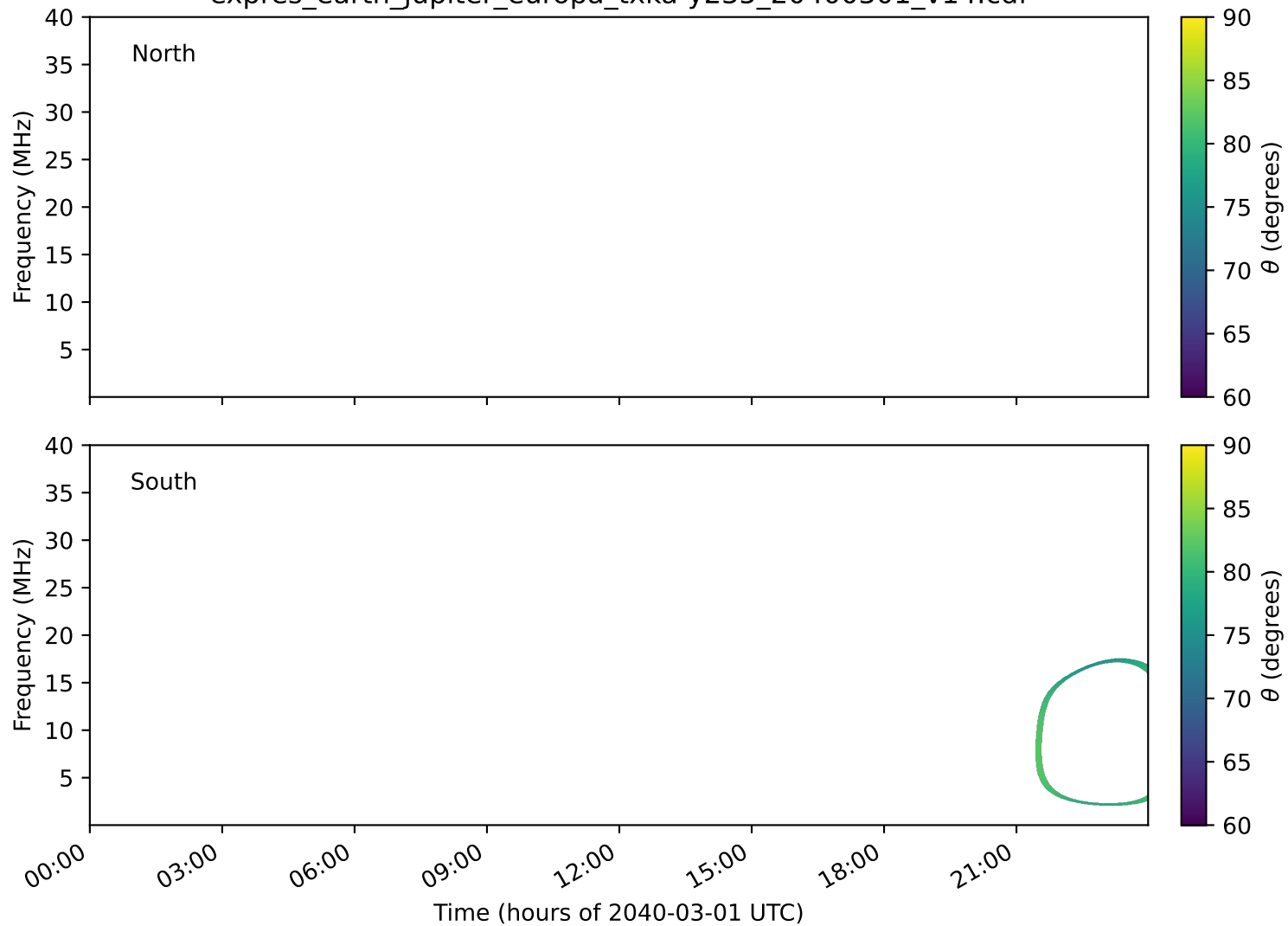
expres_earth_jupiter_europa_txka-y235_20400301_v14.cdf
