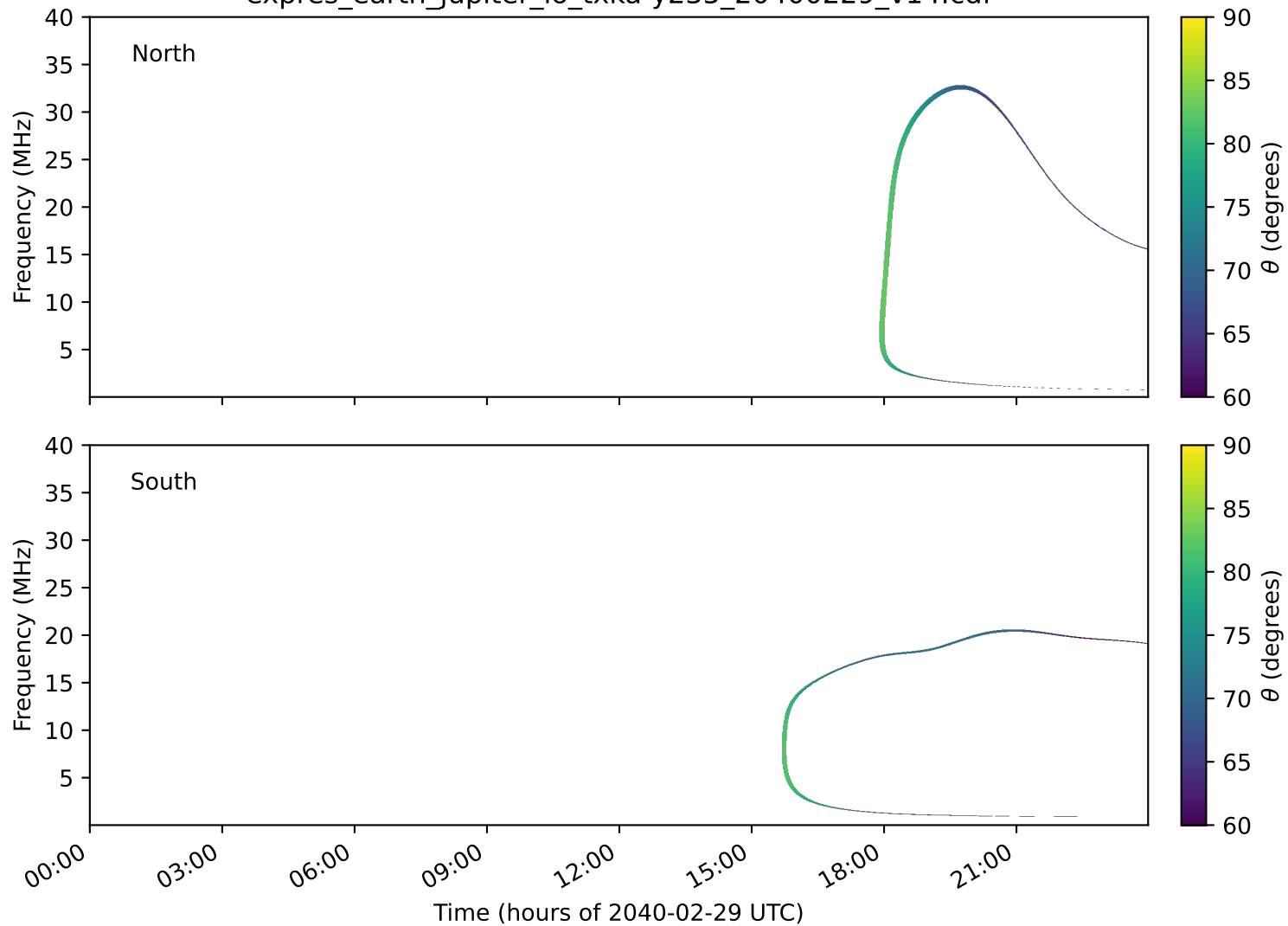
expres_earth_jupiter_io_txka-y235_20400229_v14.cdf
