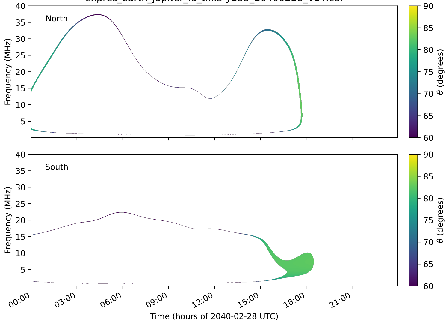
expres_earth_jupiter_io_txka-y235_20400228_v14.cdf
