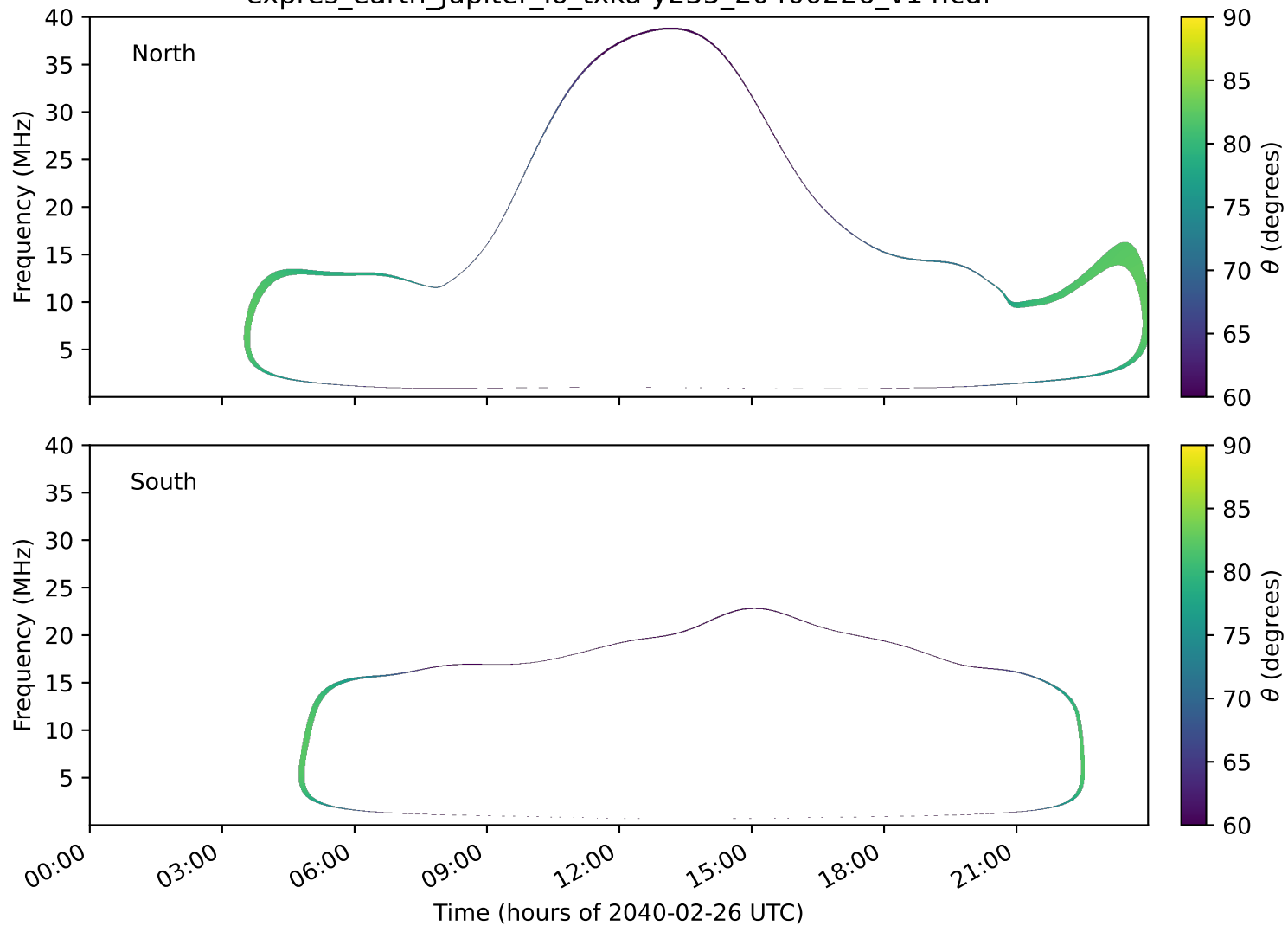
expres_earth_jupiter_io_txka-y235_20400226_v14.cdf
