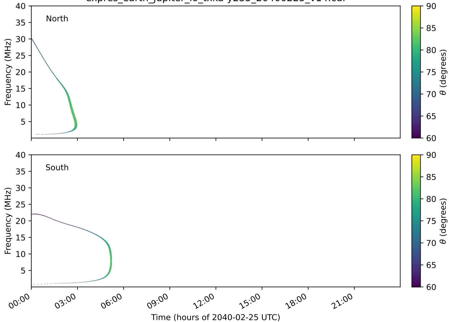
expres_earth_jupiter_io_txka-y235_20400225_v14.cdf
