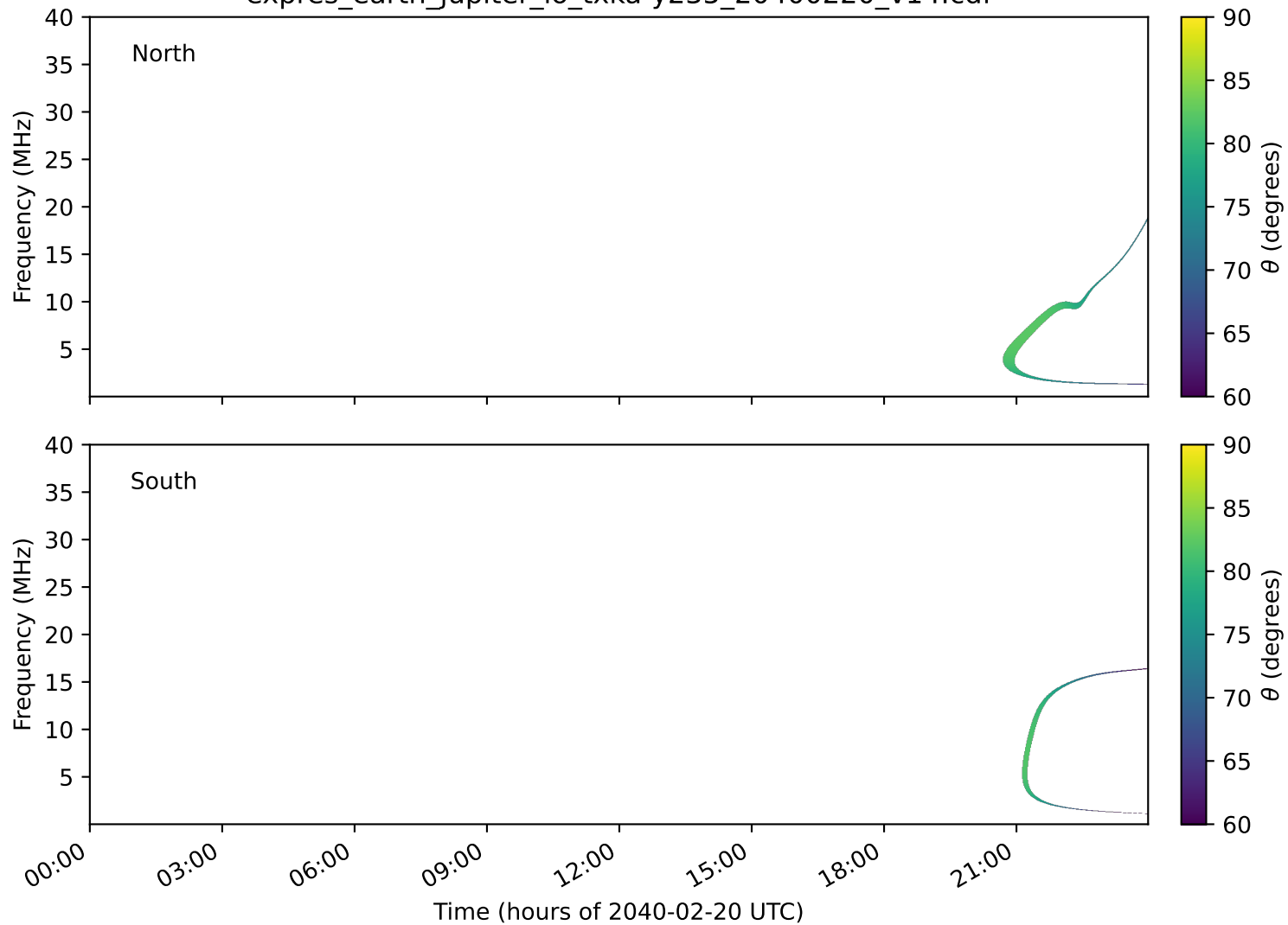
expres_earth_jupiter_io_txka-y235_20400220_v14.cdf
