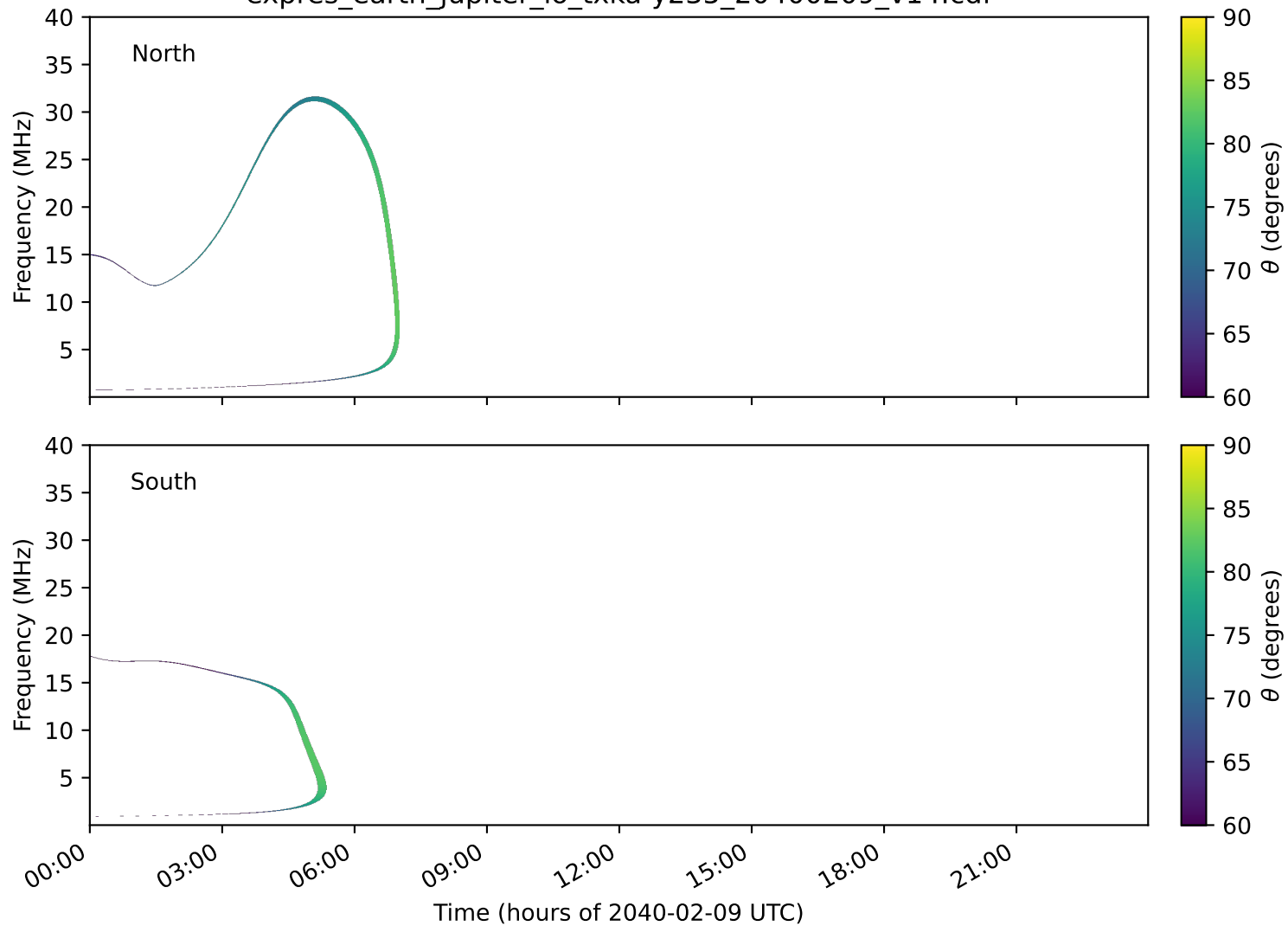
expres_earth_jupiter_io_txka-y235_20400209_v14.cdf
