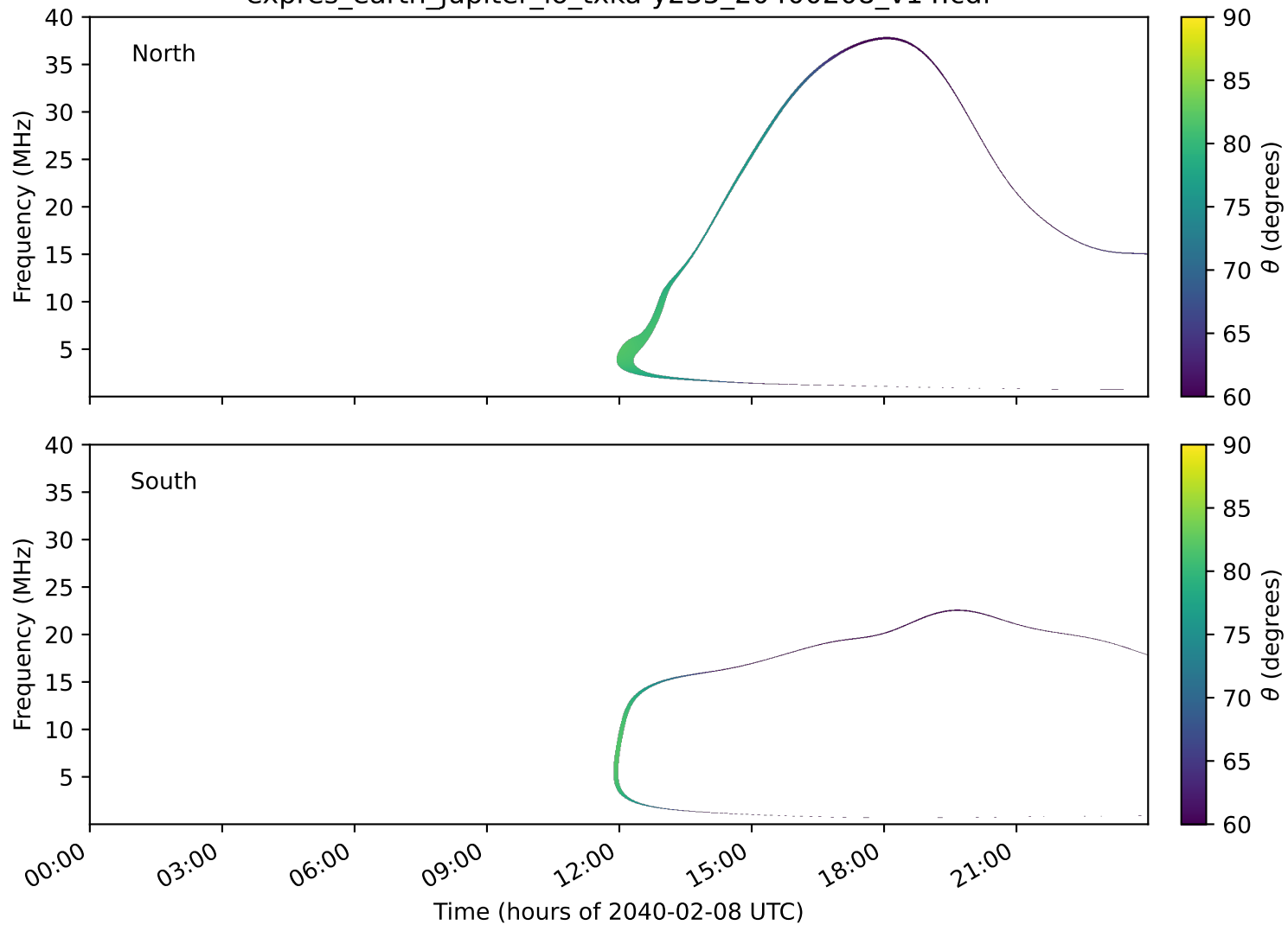
expres_earth_jupiter_io_txka-y235_20400208_v14.cdf
