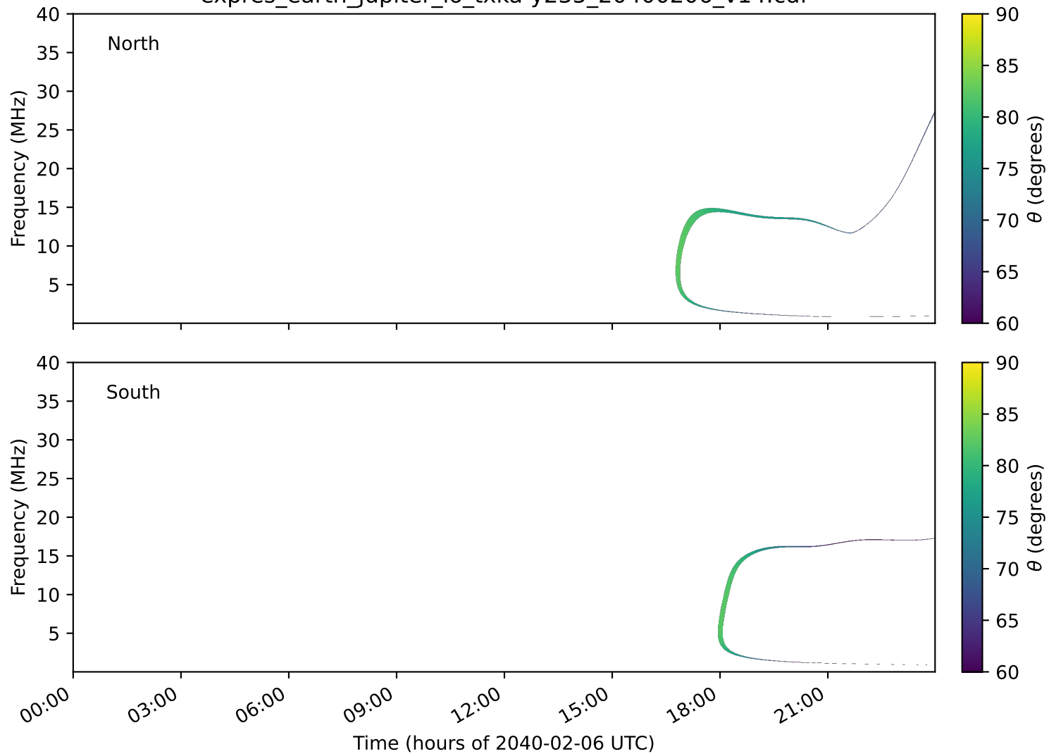
expres_earth_jupiter_io_txka-y235_20400206_v14.cdf
