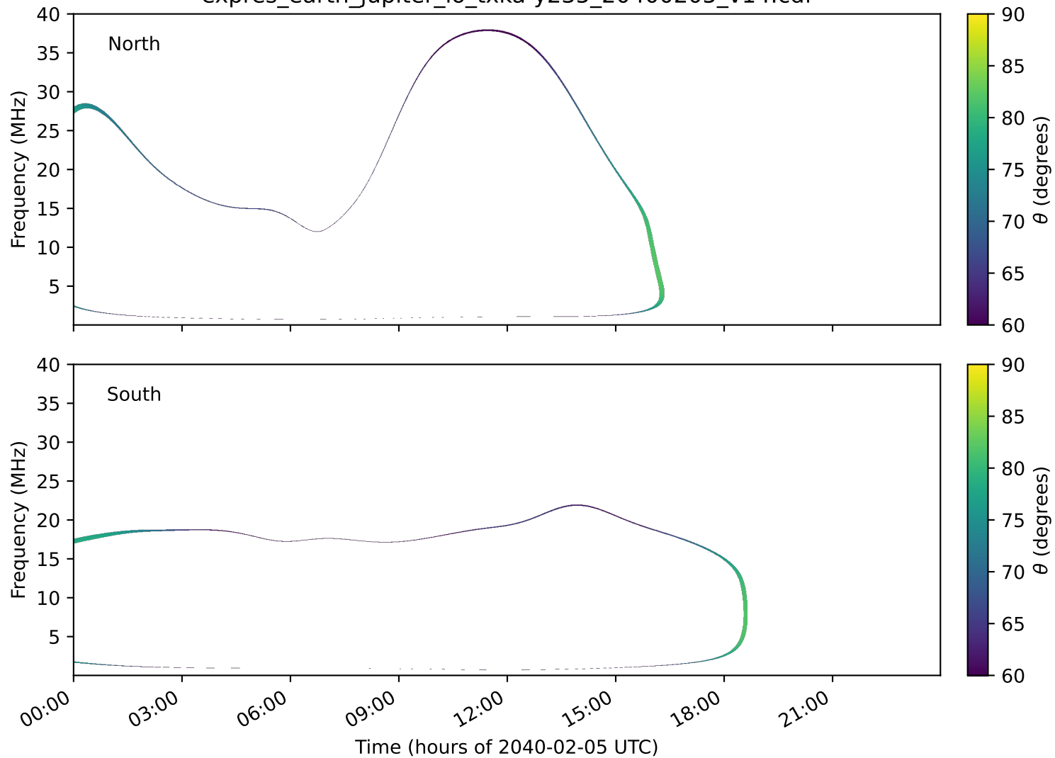
expres_earth_jupiter_io_txka-y235_20400205_v14.cdf
