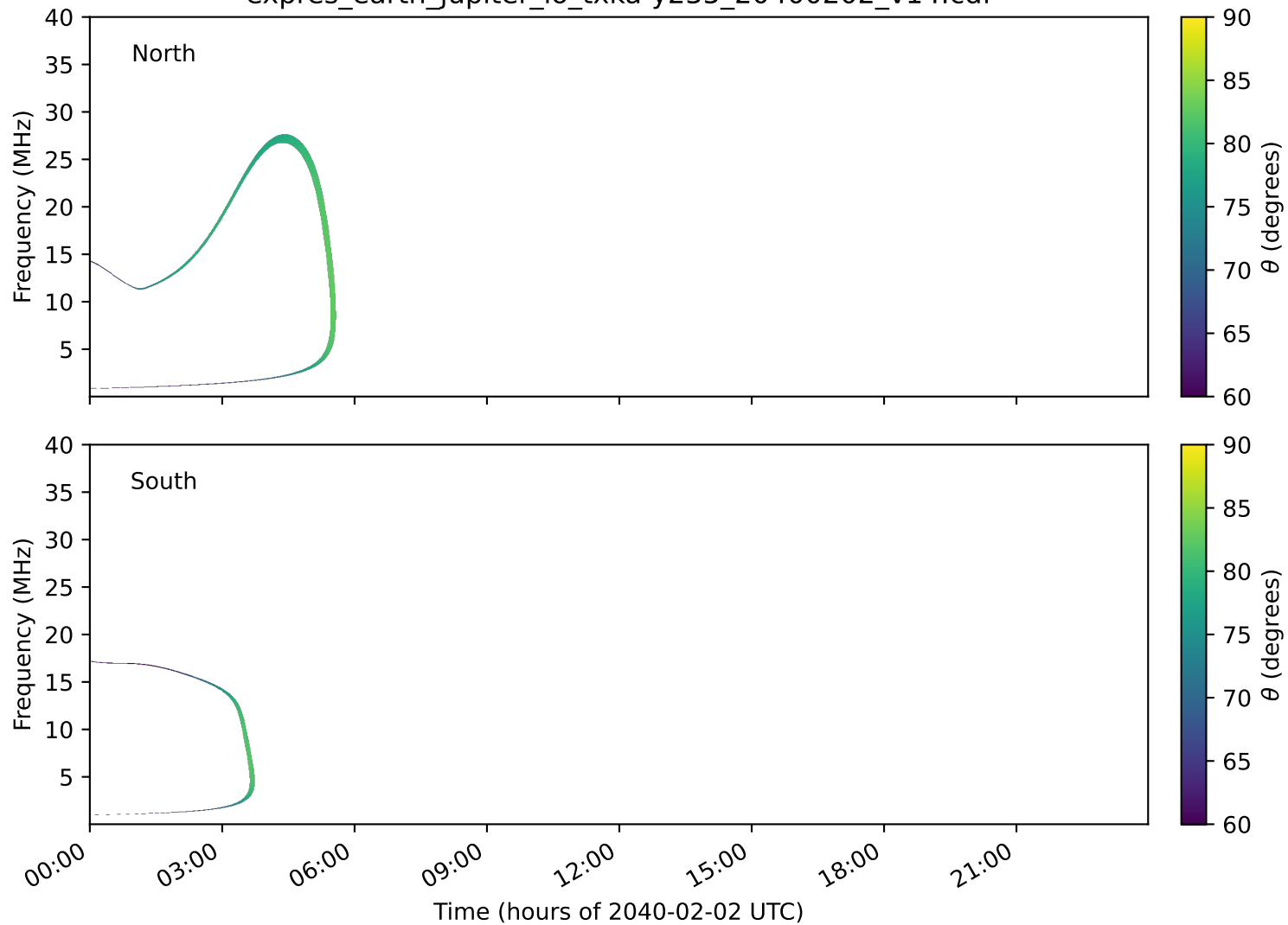
expres_earth_jupiter_io_txka-y235_20400202_v14.cdf
