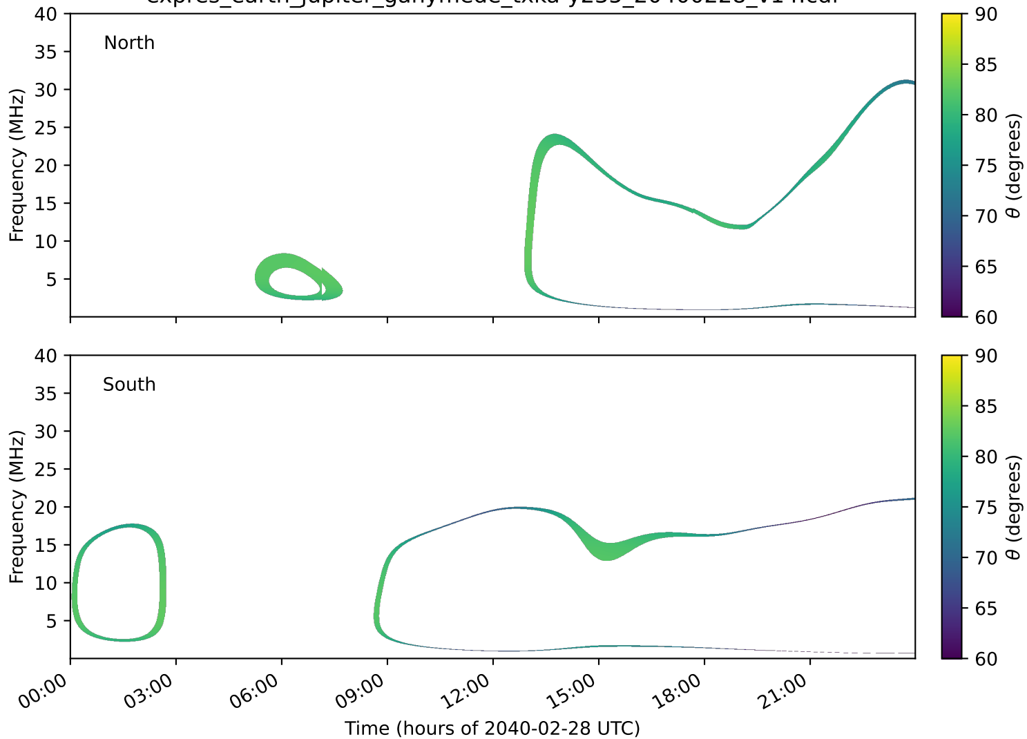
expres_earth_jupiter_ganymede_txka-y235_20400228_v14.cdf
