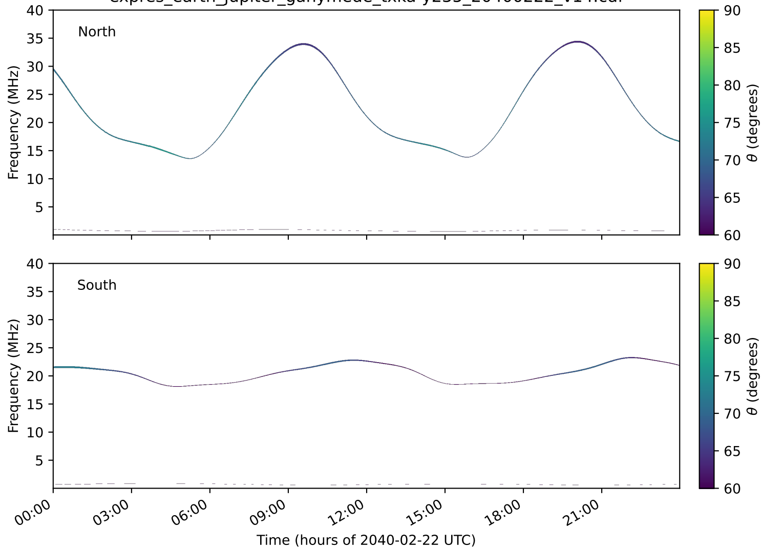
expres_earth_jupiter_ganymede_txka-y235_20400222_v14.cdf
