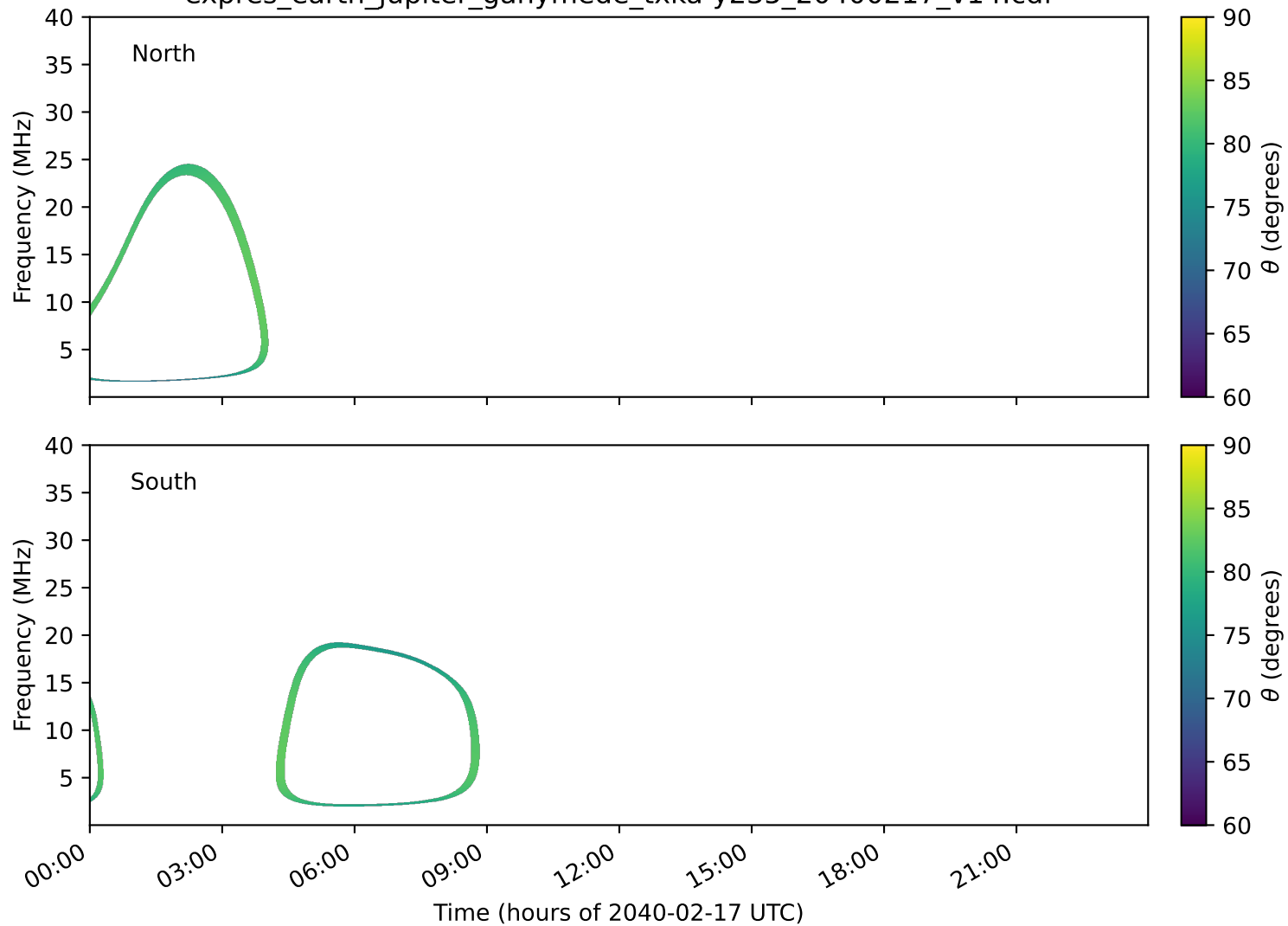
expres_earth_jupiter_ganymede_txka-y235_20400217_v14.cdf
