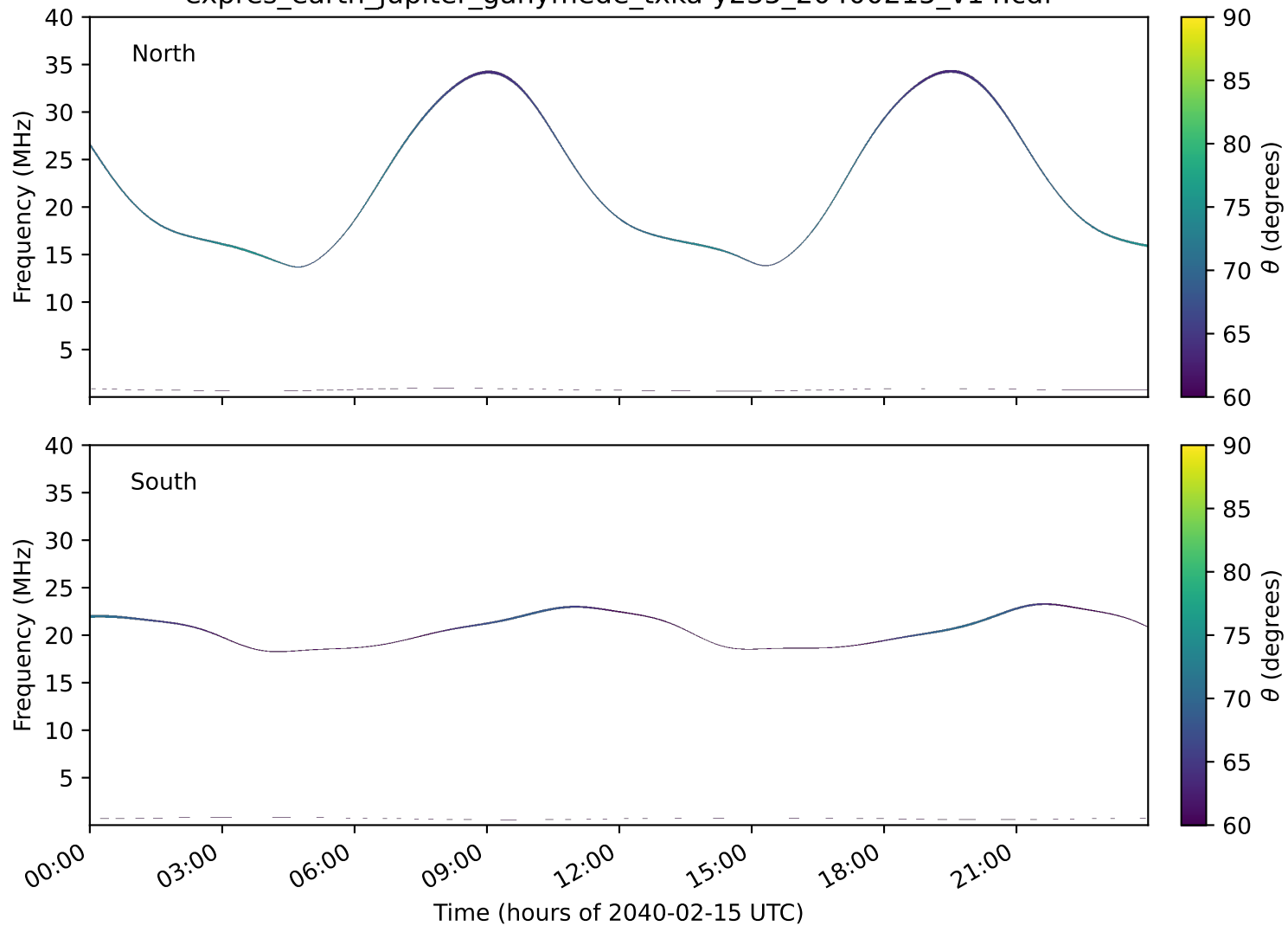
expres_earth_jupiter_ganymede_txka-y235_20400215_v14.cdf
