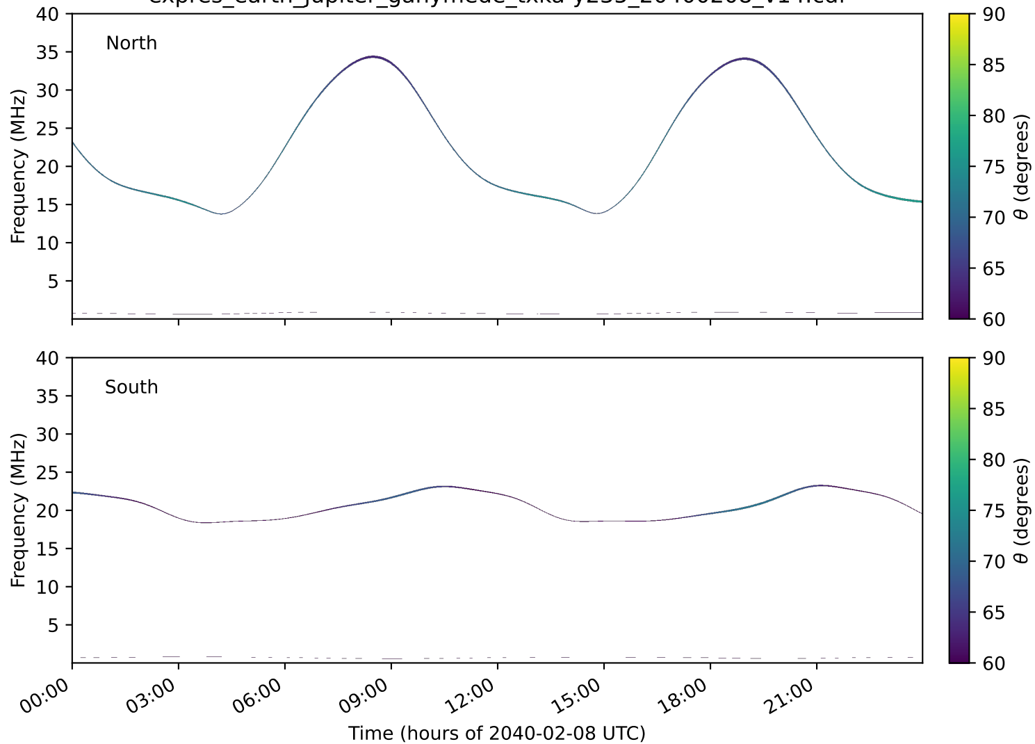
expres_earth_jupiter_ganymede_txka-y235_20400208_v14.cdf
