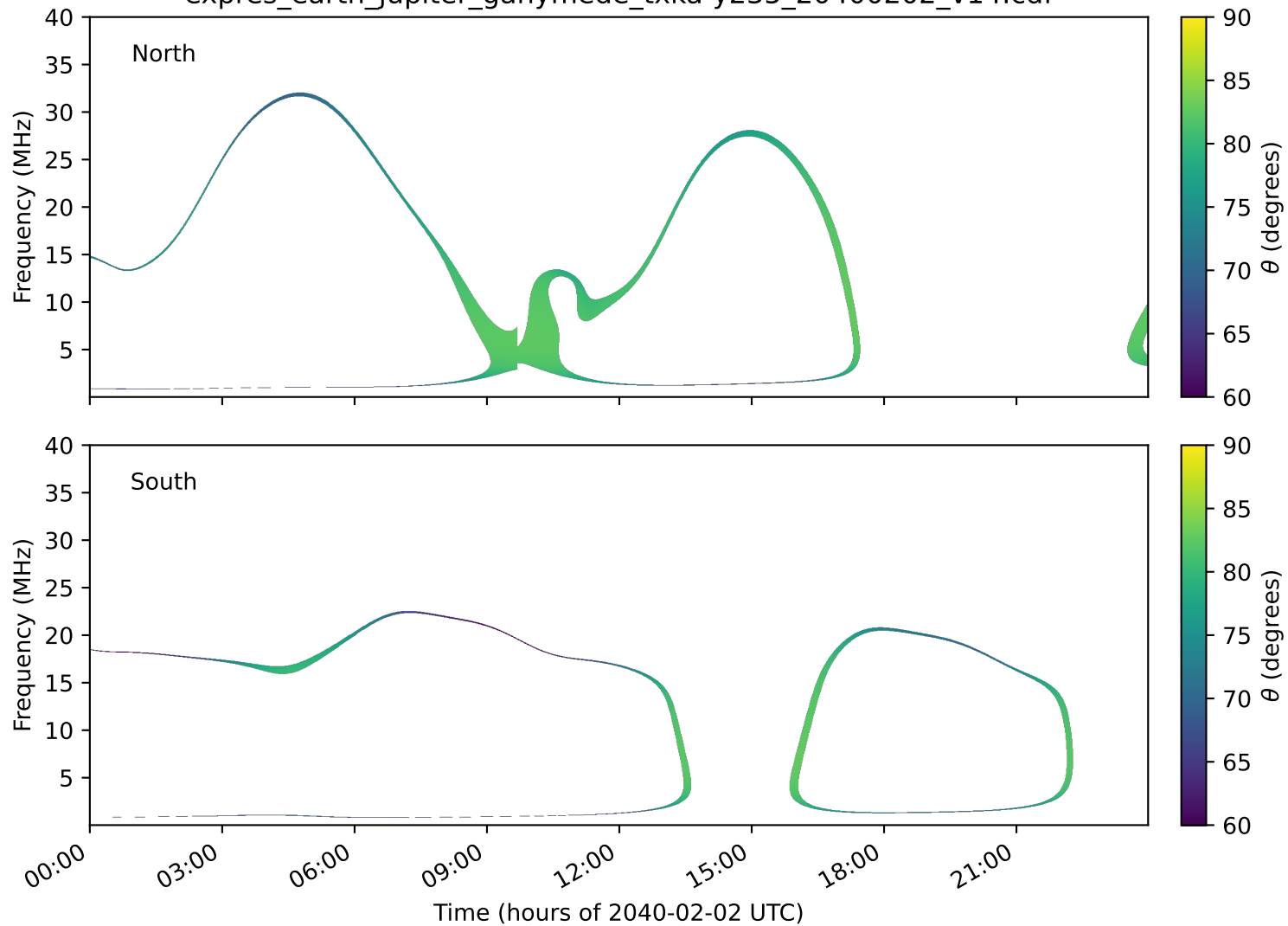
expres_earth_jupiter_ganymede_txka-y235_20400202_v14.cdf
