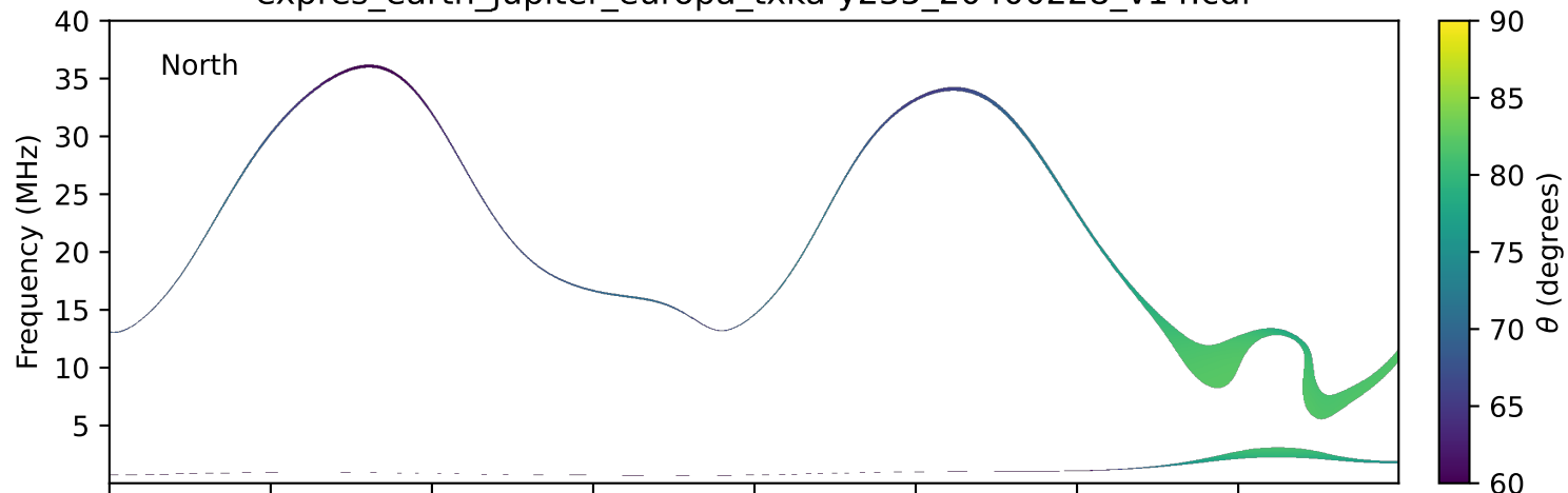
expres_earth_jupiter_europa_txka-y235_20400228_v14.cdf
