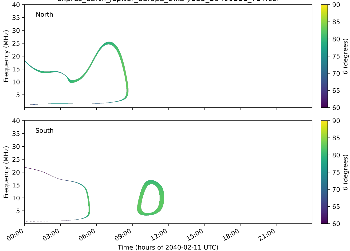
expres_earth_jupiter_europa_txka-y235_20400211_v14.cdf
