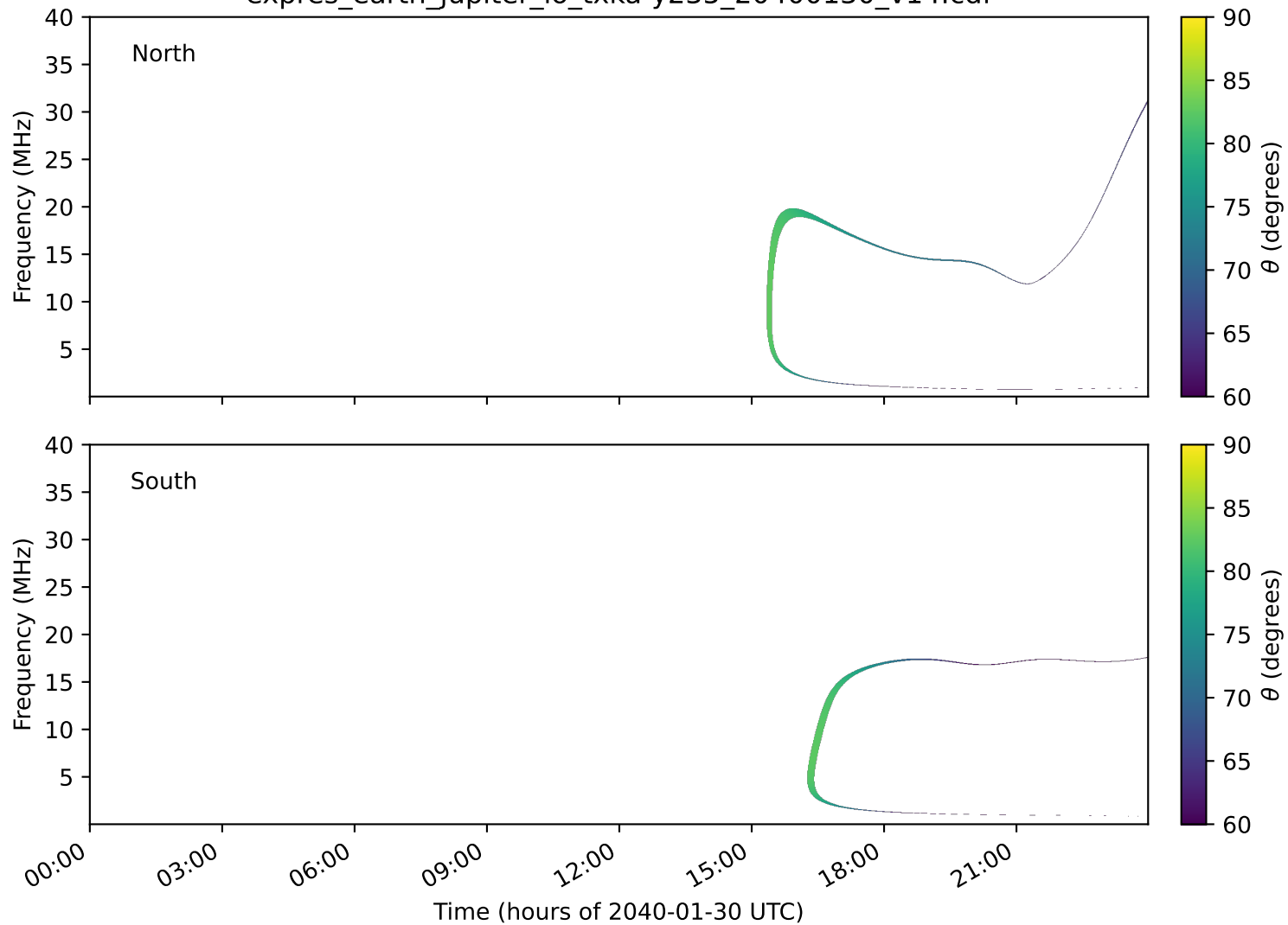
expres_earth_jupiter_io_txka-y235_20400130_v14.cdf
