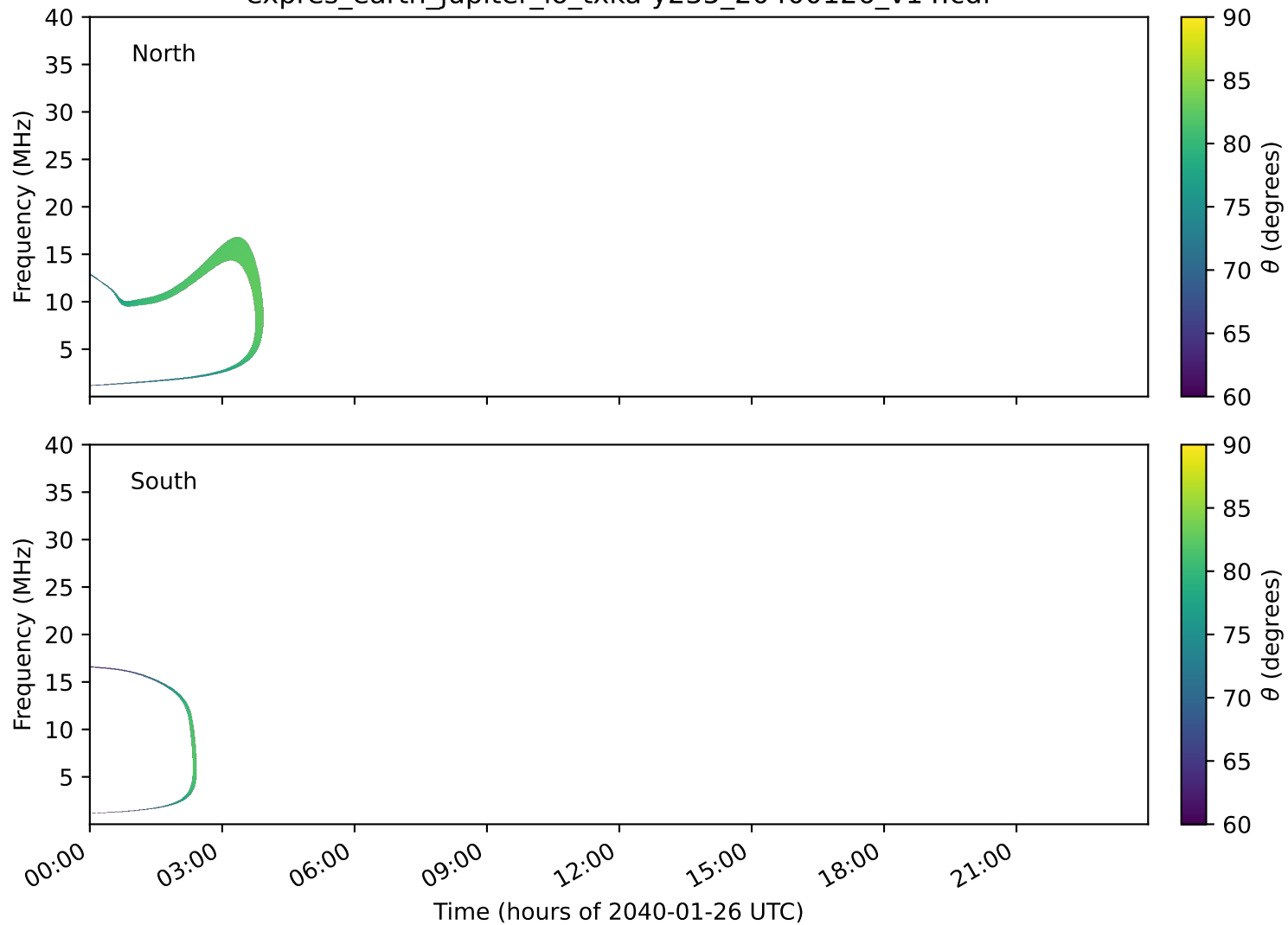
expres_earth_jupiter_io_txka-y235_20400126_v14.cdf
