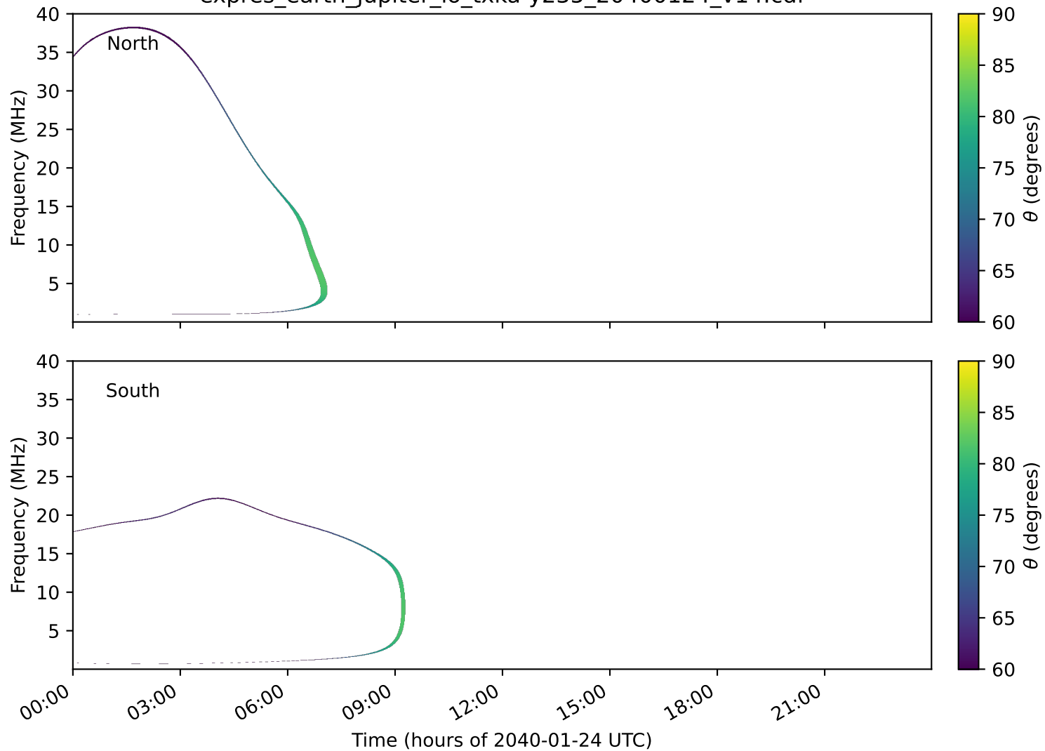
expres_earth_jupiter_io_txka-y235_20400124_v14.cdf
