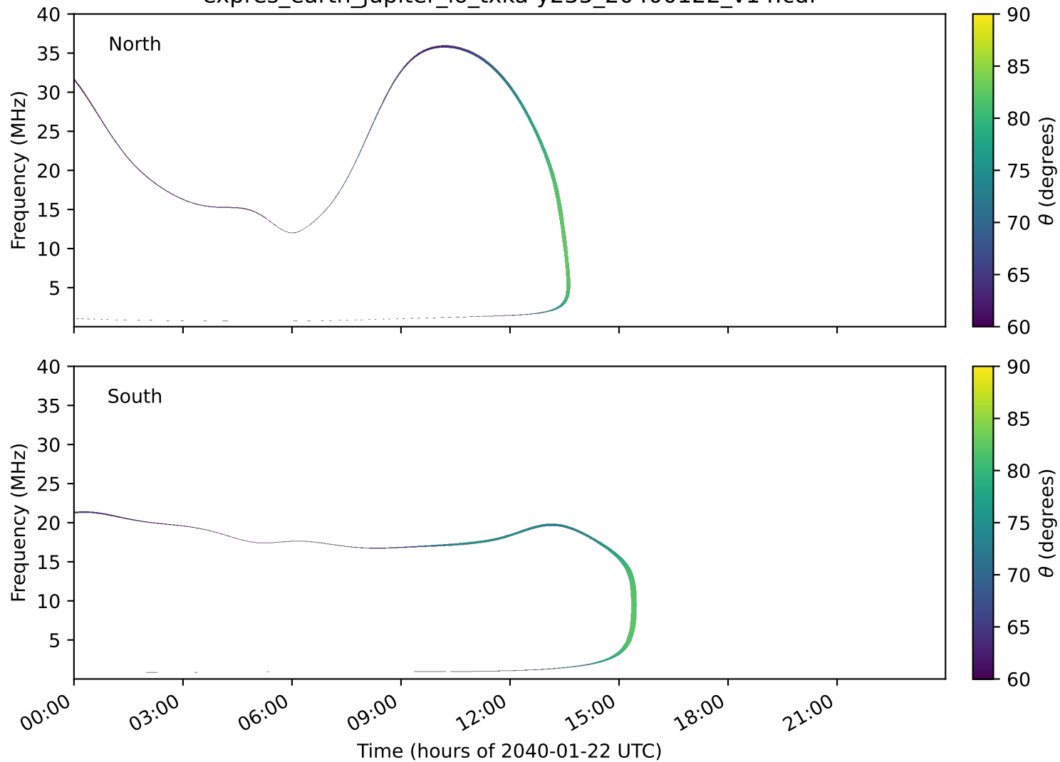
expres_earth_jupiter_io_txka-y235_20400122_v14.cdf
