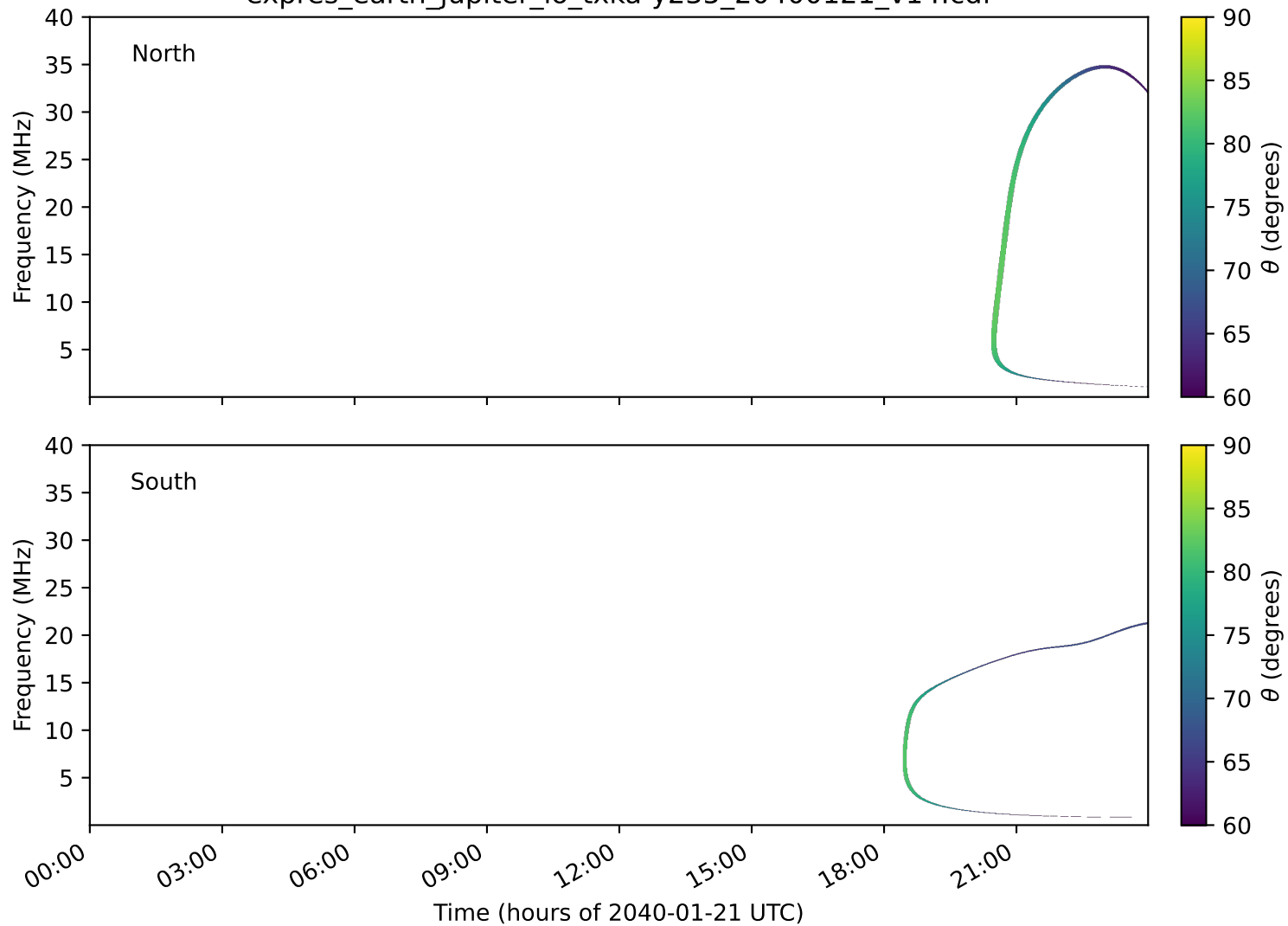
expres_earth_jupiter_io_txka-y235_20400121_v14.cdf
