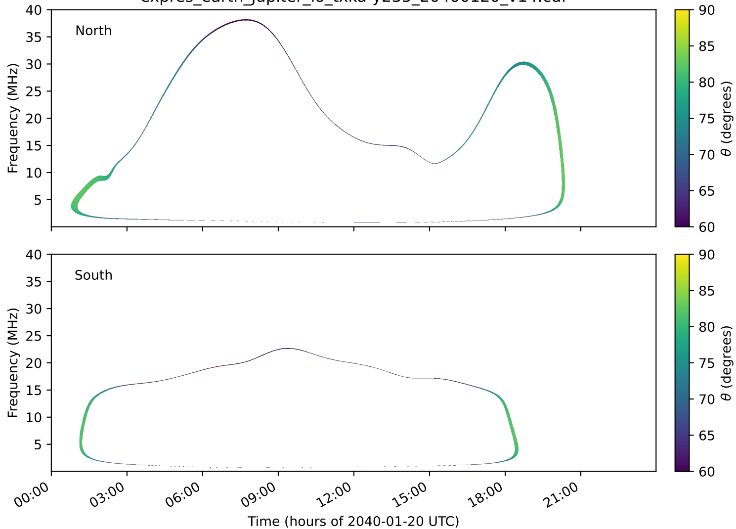
expres_earth_jupiter_io_txka-y235_20400120_v14.cdf
