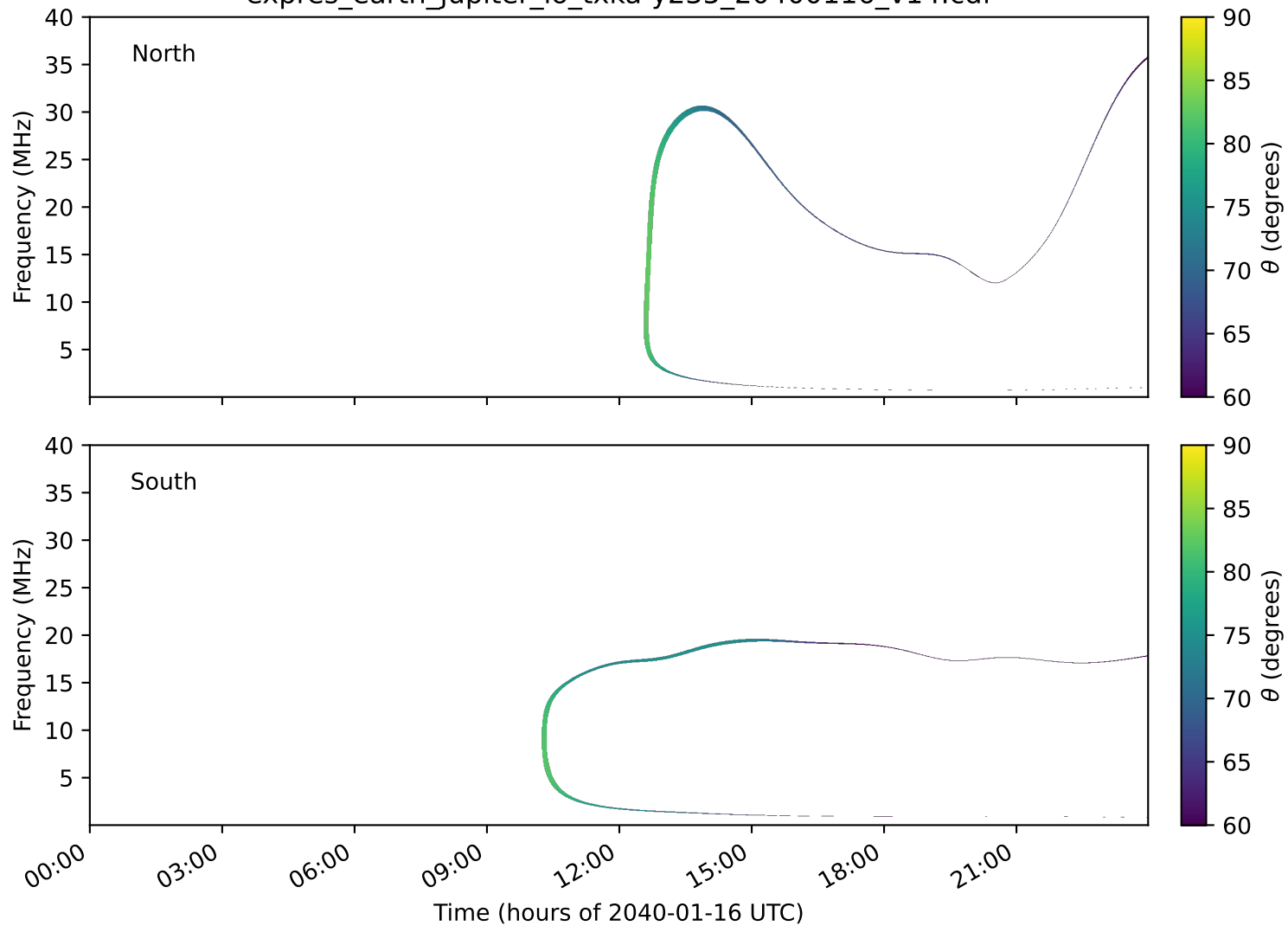
expres_earth_jupiter_io_txka-y235_20400116_v14.cdf
