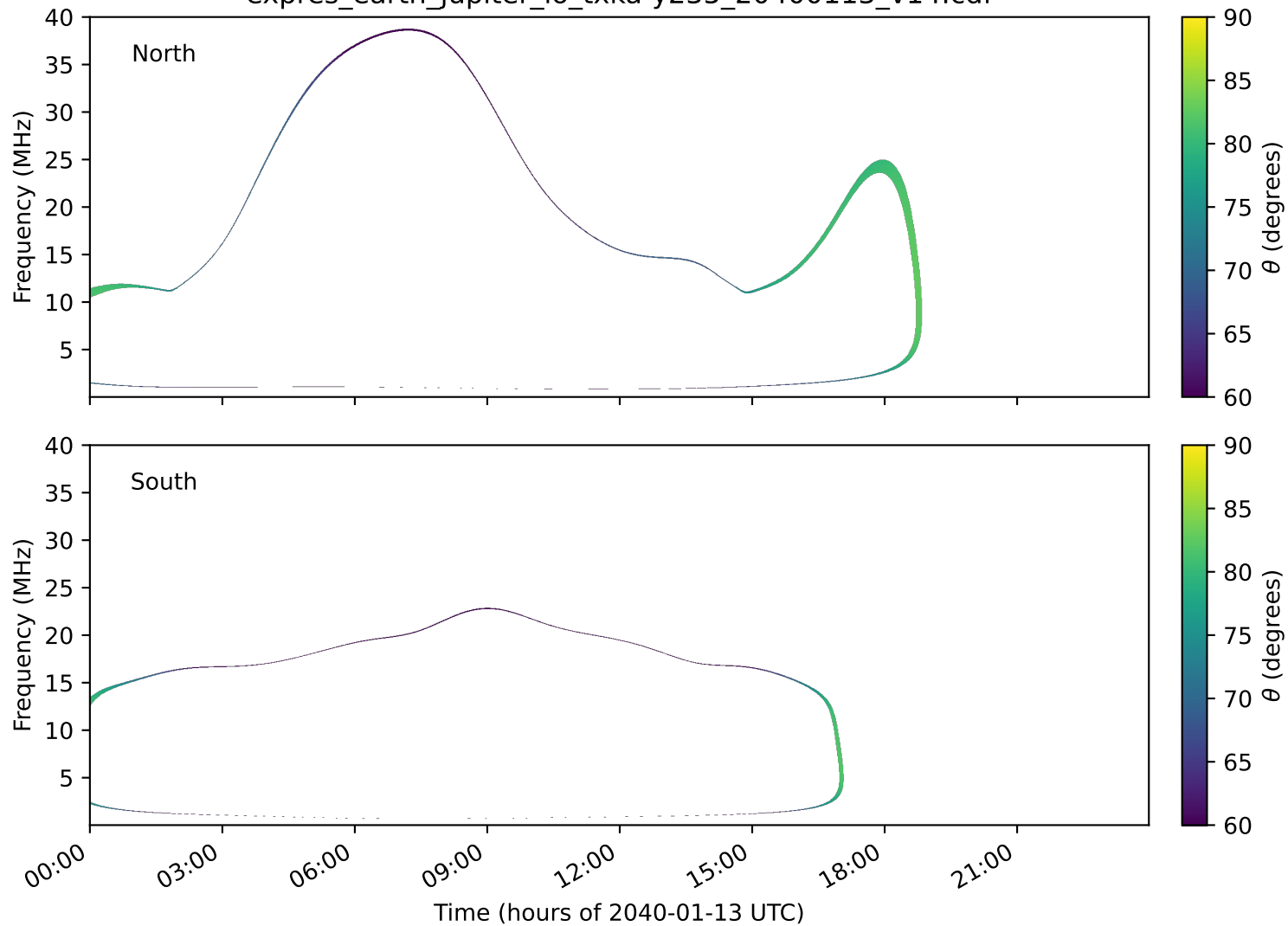
expres_earth_jupiter_io_txka-y235_20400113_v14.cdf
