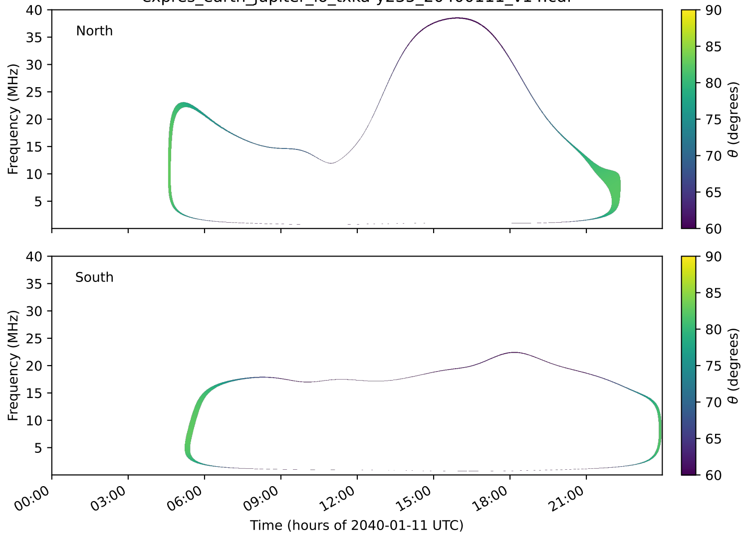
expres_earth_jupiter_io_txka-y235_20400111_v14.cdf
