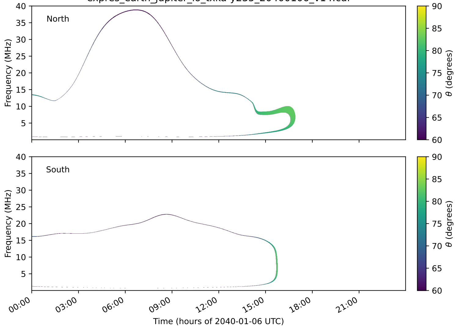
expres_earth_jupiter_io_txka-y235_20400106_v14.cdf
