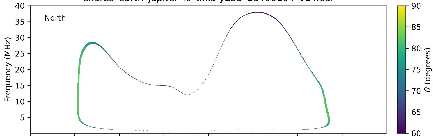
expres_earth_jupiter_io_txka-y235_20400104_v14.cdf
