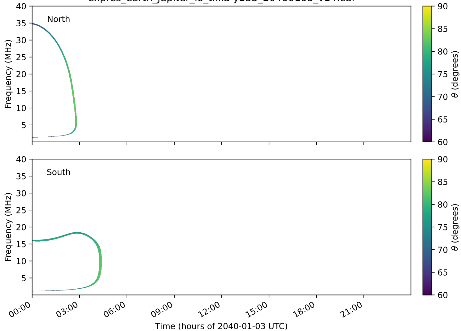
expres_earth_jupiter_io_txka-y235_20400103_v14.cdf
