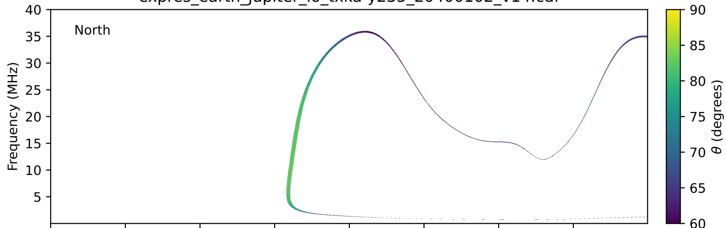
expres_earth_jupiter_io_txka-y235_20400102_v14.cdf
