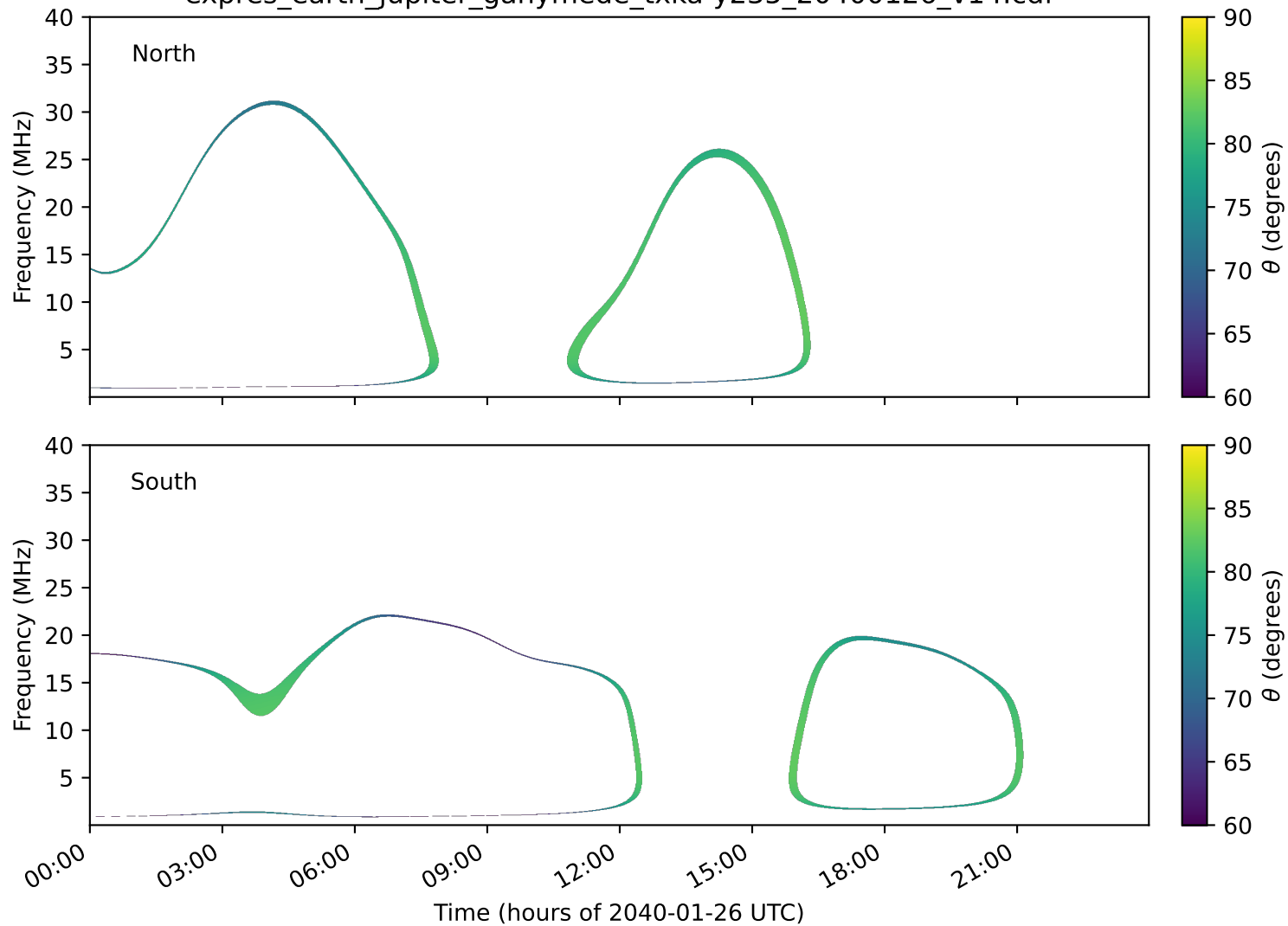
expres_earth_jupiter_ganymede_txka-y235_20400126_v14.cdf
