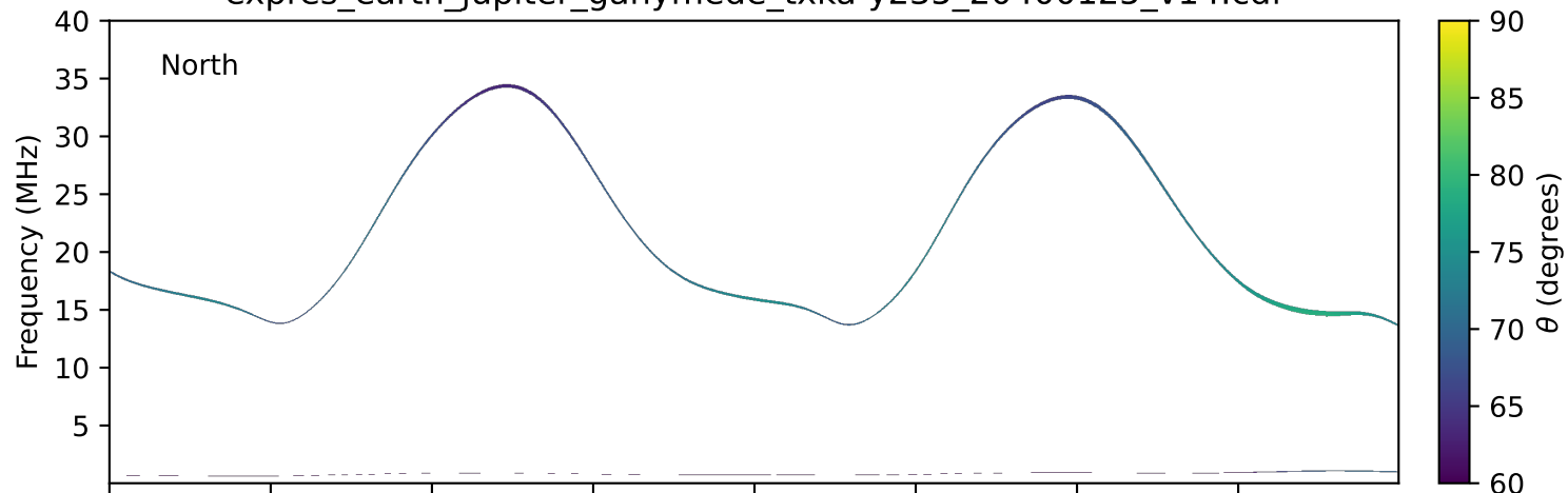
expres_earth_jupiter_ganymede_txka-y235_20400125_v14.cdf
