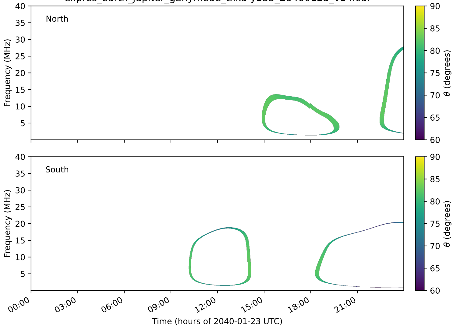
expres_earth_jupiter_ganymede_txka-y235_20400123_v14.cdf
