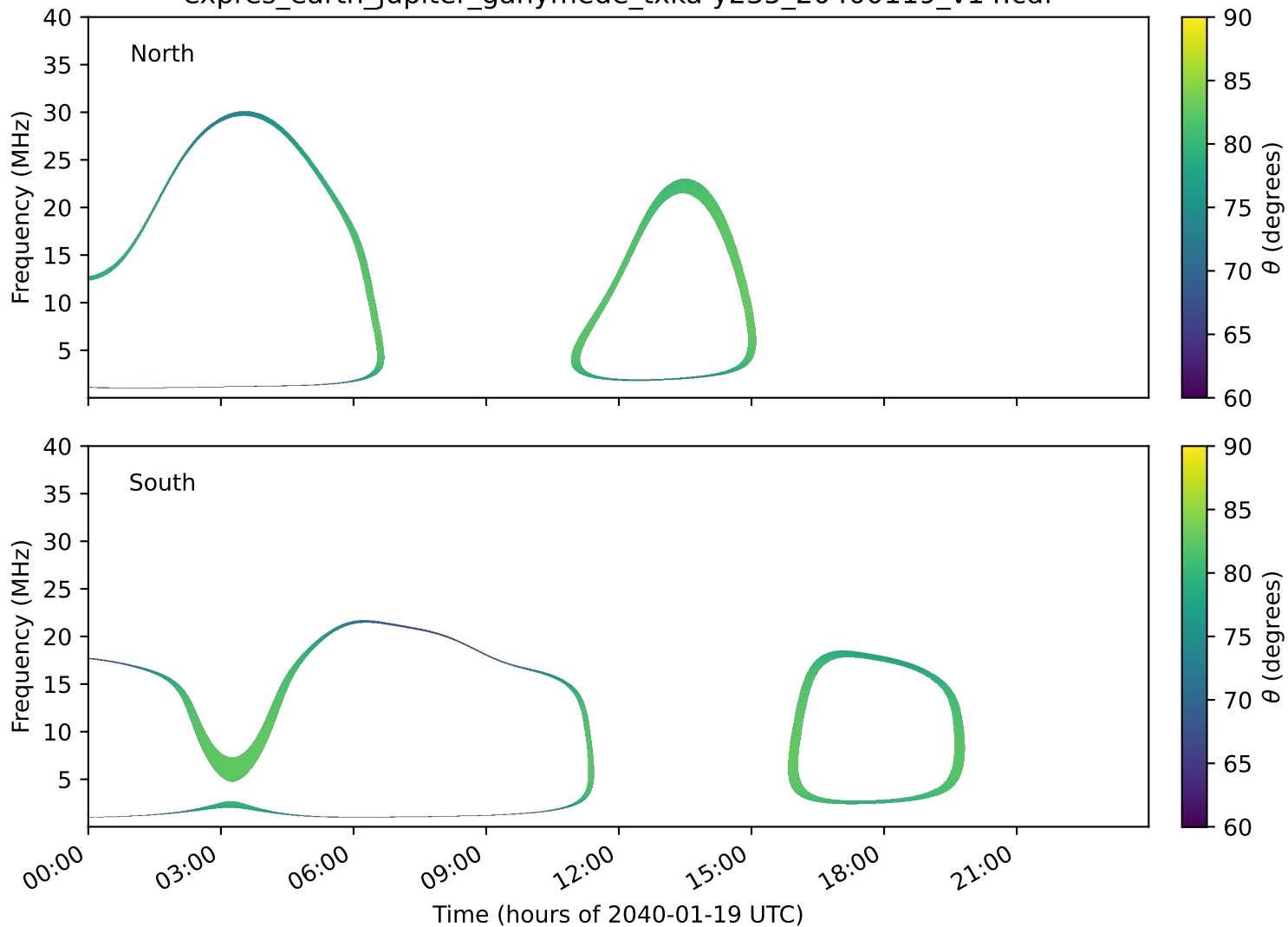
expres_earth_jupiter_ganymede_txka-y235_20400119_v14.cdf
