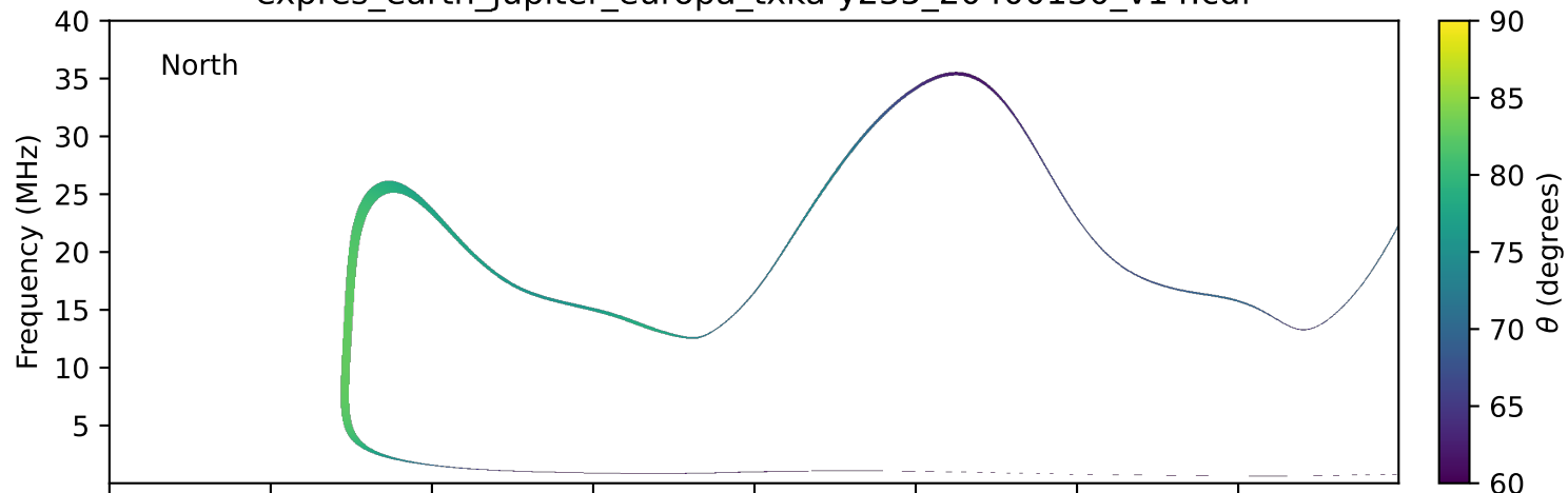
expres_earth_jupiter_europa_txka-y235_20400130_v14.cdf
