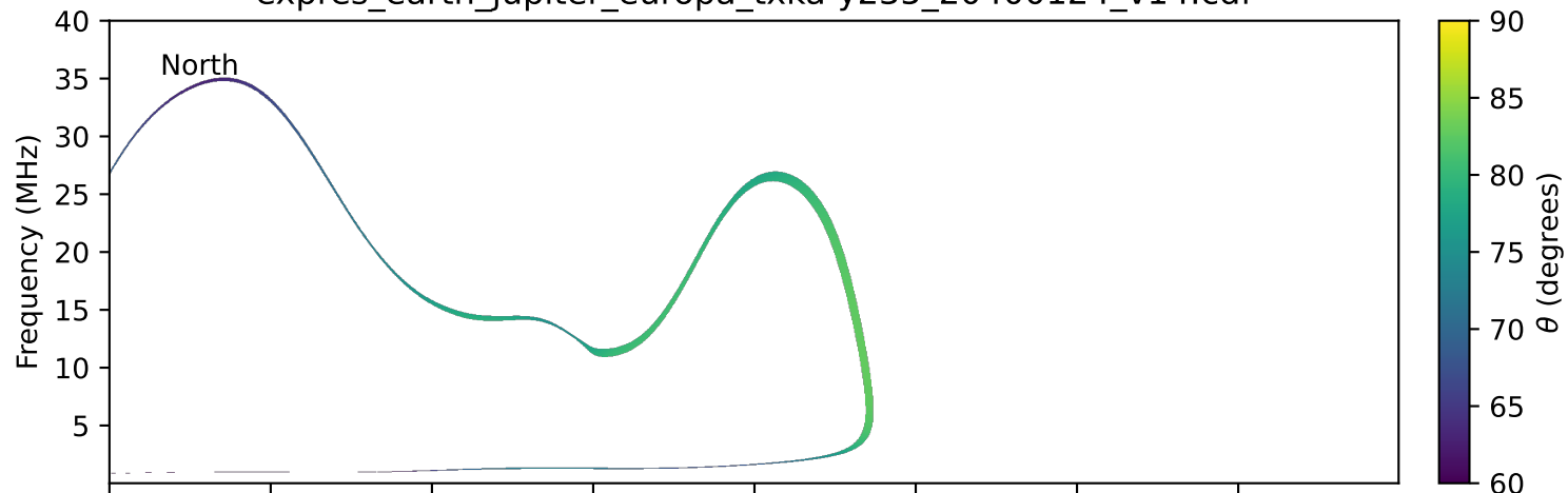
expres_earth_jupiter_europa_txka-y235_20400124_v14.cdf
