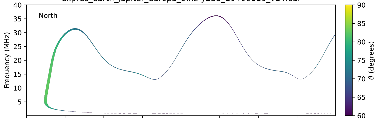
expres_earth_jupiter_europa_txka-y235_20400116_v14.cdf
