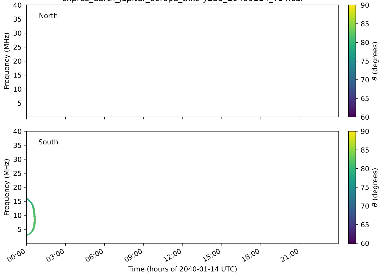
expres_earth_jupiter_europa_txka-y235_20400114_v14.cdf
