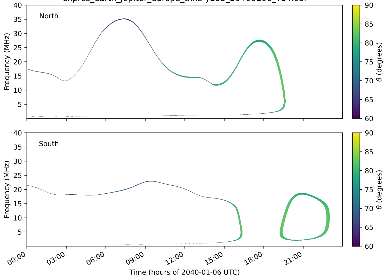
expres_earth_jupiter_europa_txka-y235_20400106_v14.cdf
