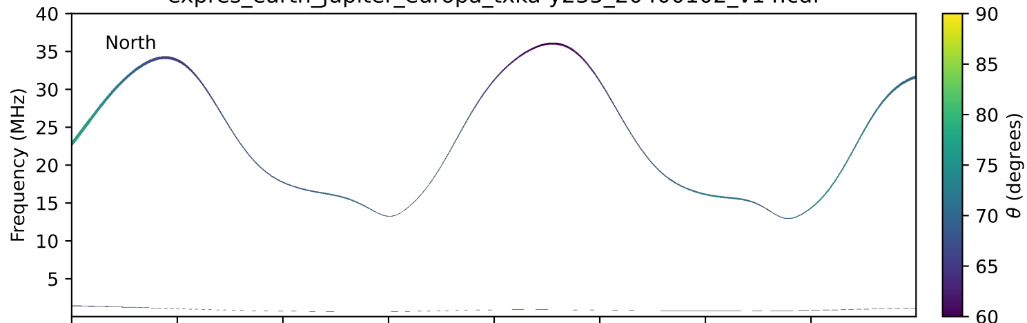
expres_earth_jupiter_europa_txka-y235_20400102_v14.cdf
