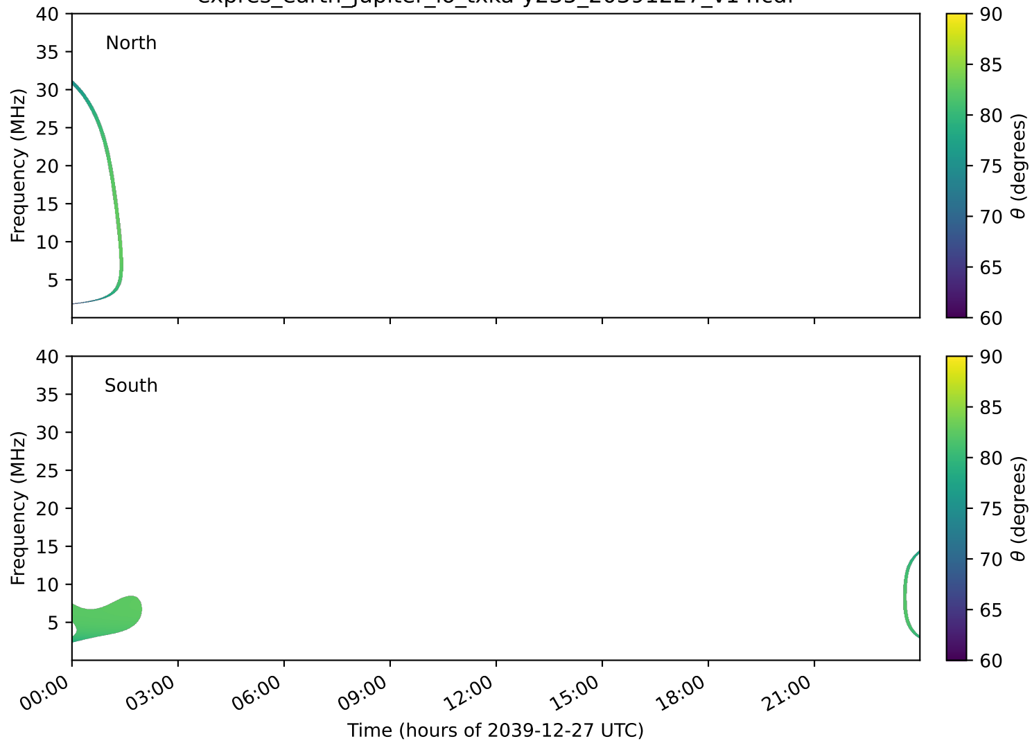
expres_earth_jupiter_io_txka-y235_20391227_v14.cdf
