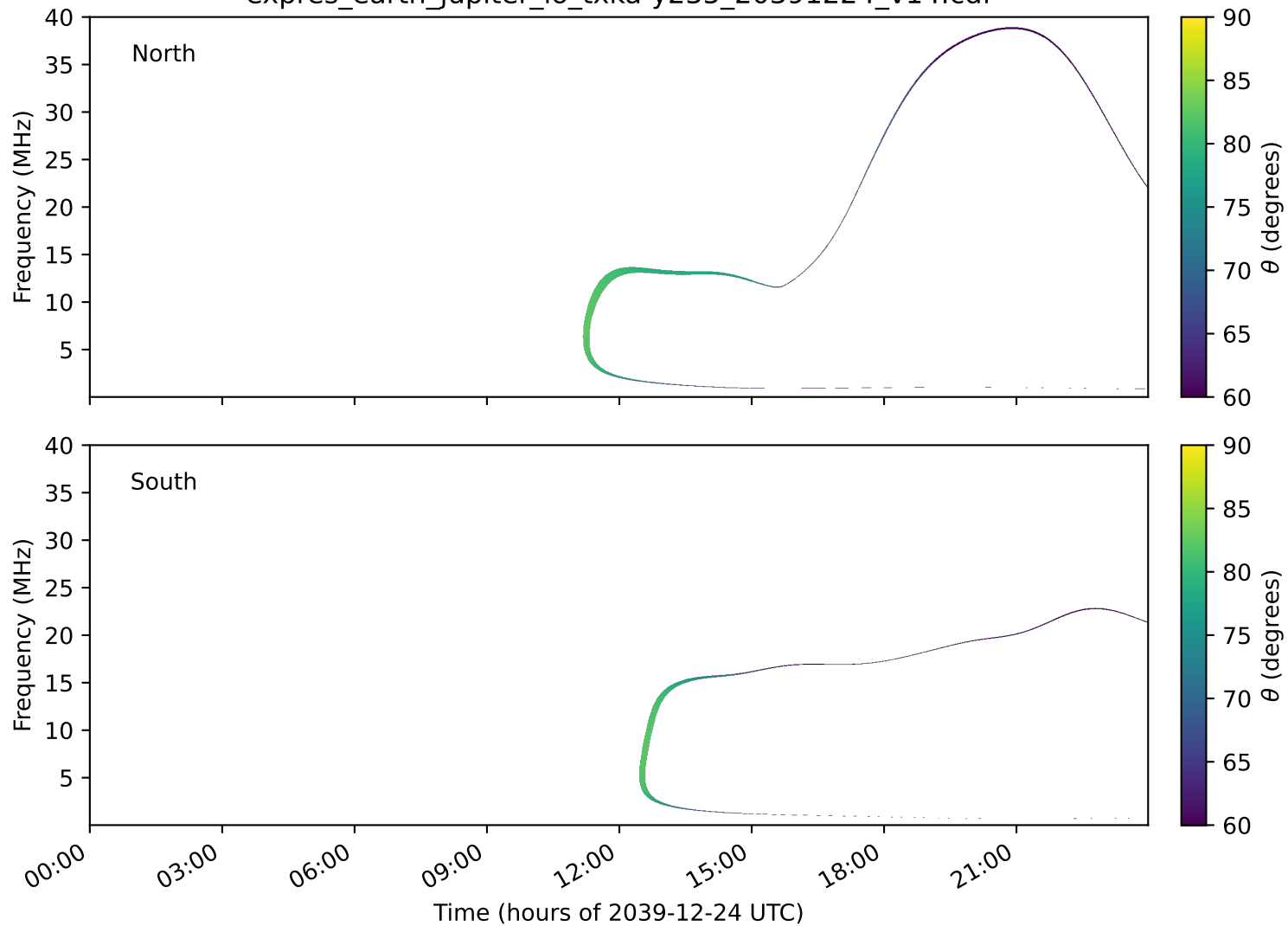
expres_earth_jupiter_io_txka-y235_20391224_v14.cdf
