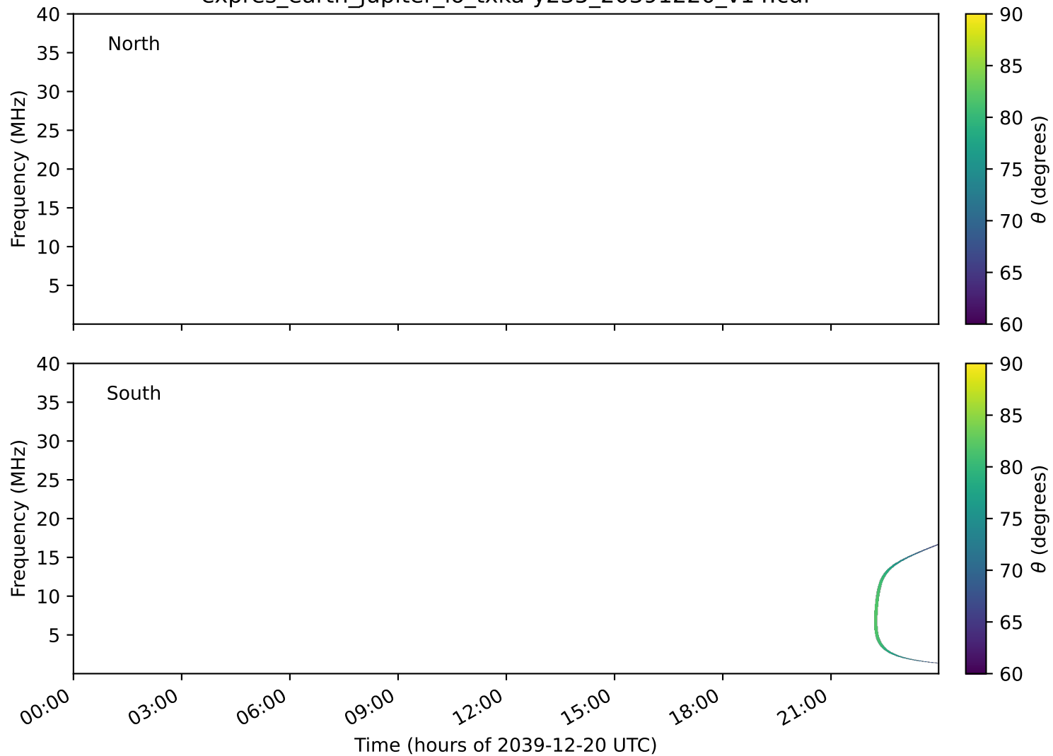
expres_earth_jupiter_io_txka-y235_20391220_v14.cdf
