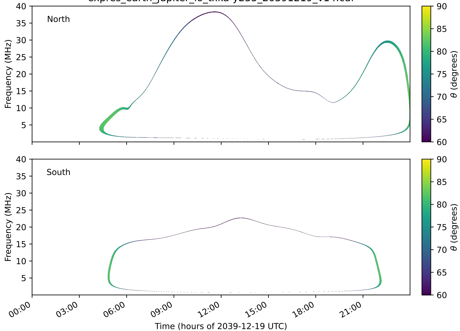
expres_earth_jupiter_io_txka-y235_20391219_v14.cdf
