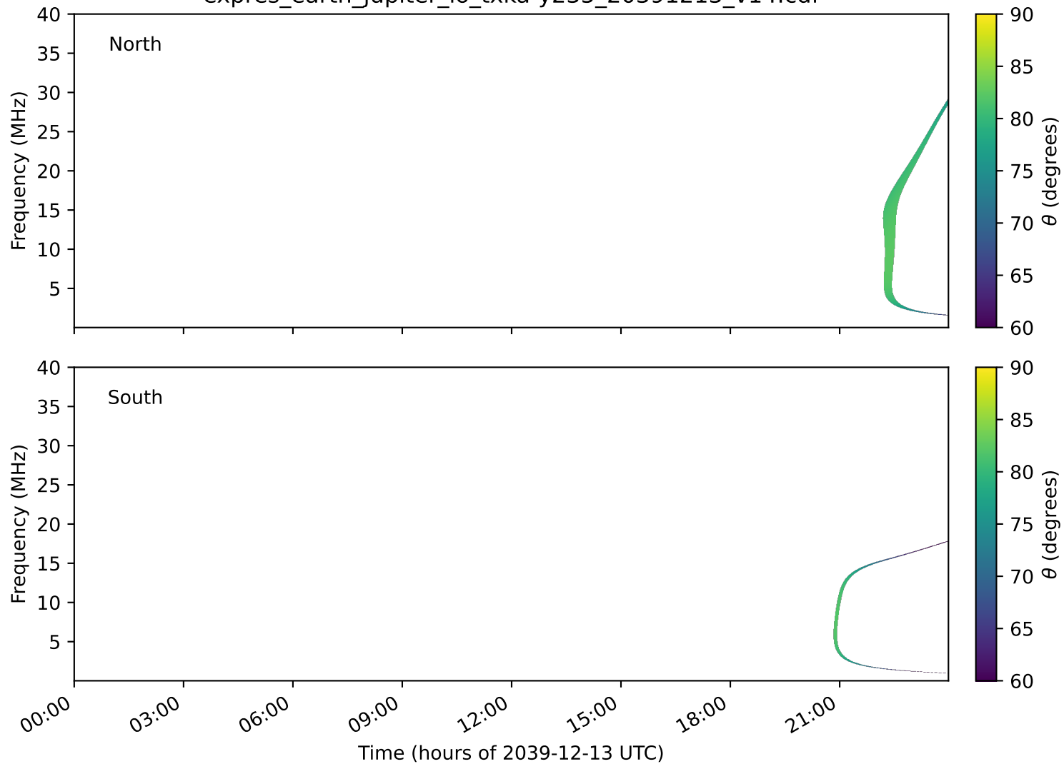
expres_earth_jupiter_io_txka-y235_20391213_v14.cdf
