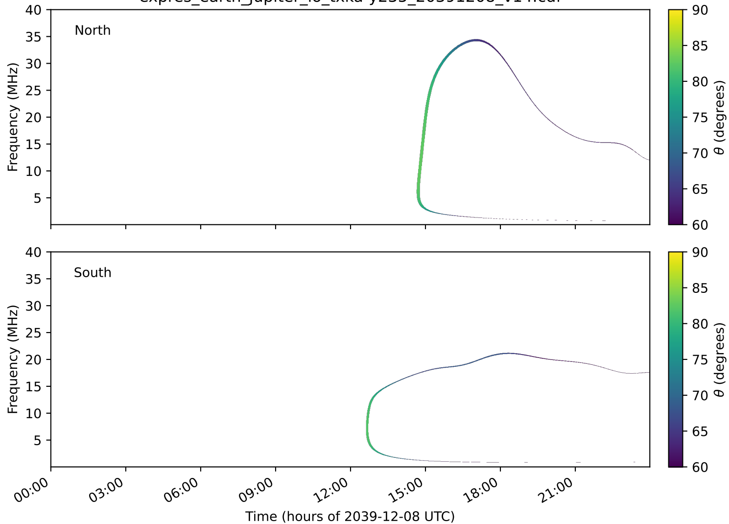
expres_earth_jupiter_io_txka-y235_20391208_v14.cdf
