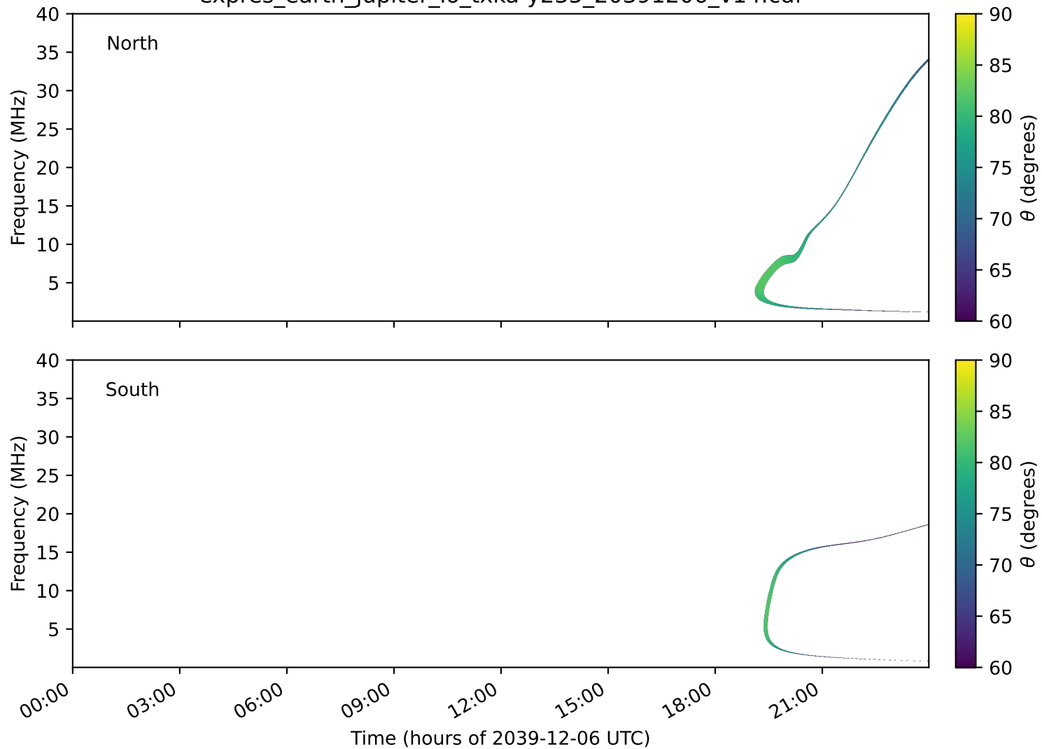
expres_earth_jupiter_io_txka-y235_20391206_v14.cdf
