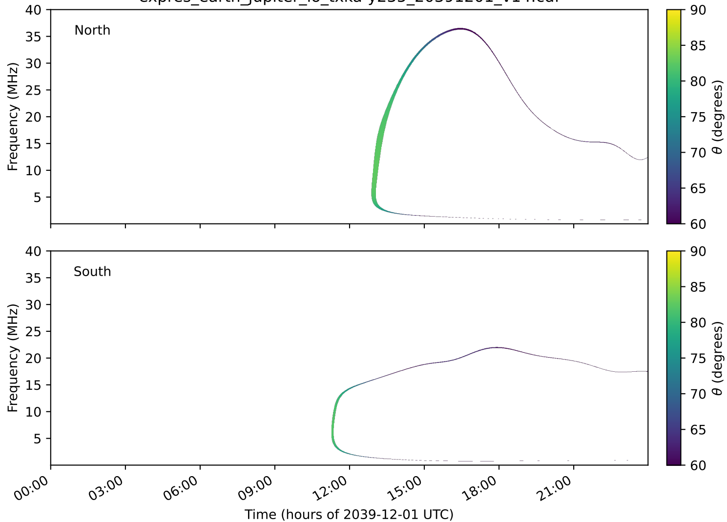
expres_earth_jupiter_io_txka-y235_20391201_v14.cdf
